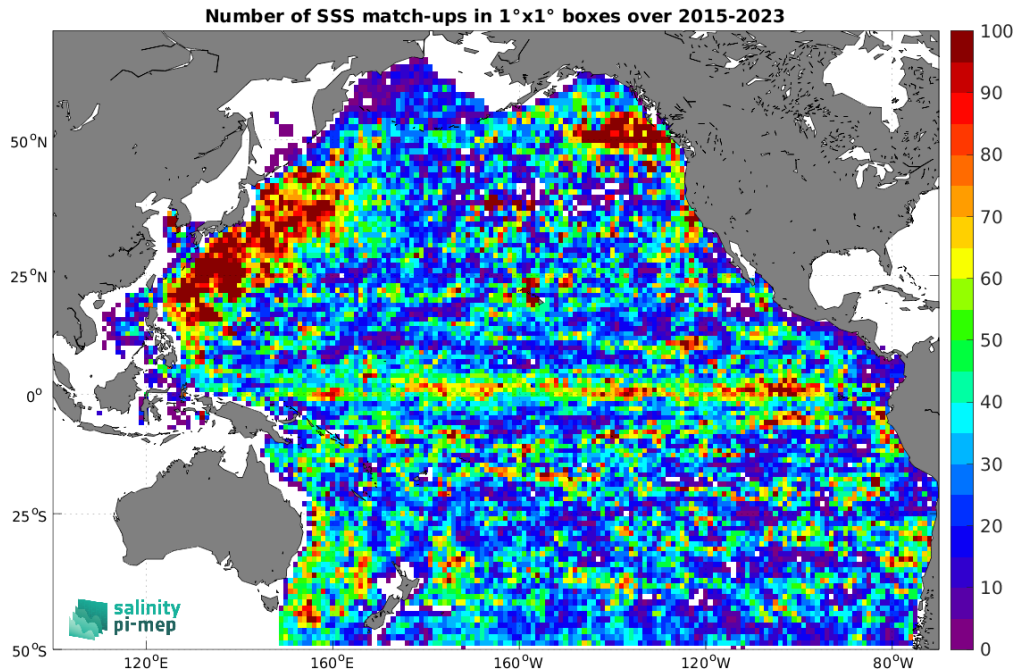
Figure 5: Number of SSS match-ups between Argo SSS and the SMAP SSS L3 v5.3 - 8-Day running (RSS) SSS product for the Pacific Ocean Pi-MEP region over 1^\circ \times 1^\circ boxes and for the full satellite product period.
