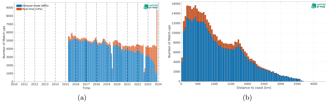
Figure 2: Number of match-ups between Argo and SMAP SSS L3 v5.3 - 8-Day running (RSS) SSS as a function of time (a) and as function of the distance to coast (b) over the Pacific Ocean Pi-MEP region and for the full satellite product period.
