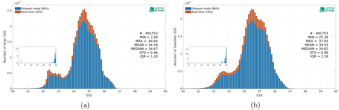
Figure 3: Histograms of SSS from Argo (a) and SMAP SSS L3 v5.3 - 8-Day running (RSS) (b) considering all match-up pairs per bins of 0.1 over the Pacific Ocean Pi-MEP region and for the full satellite product period.
