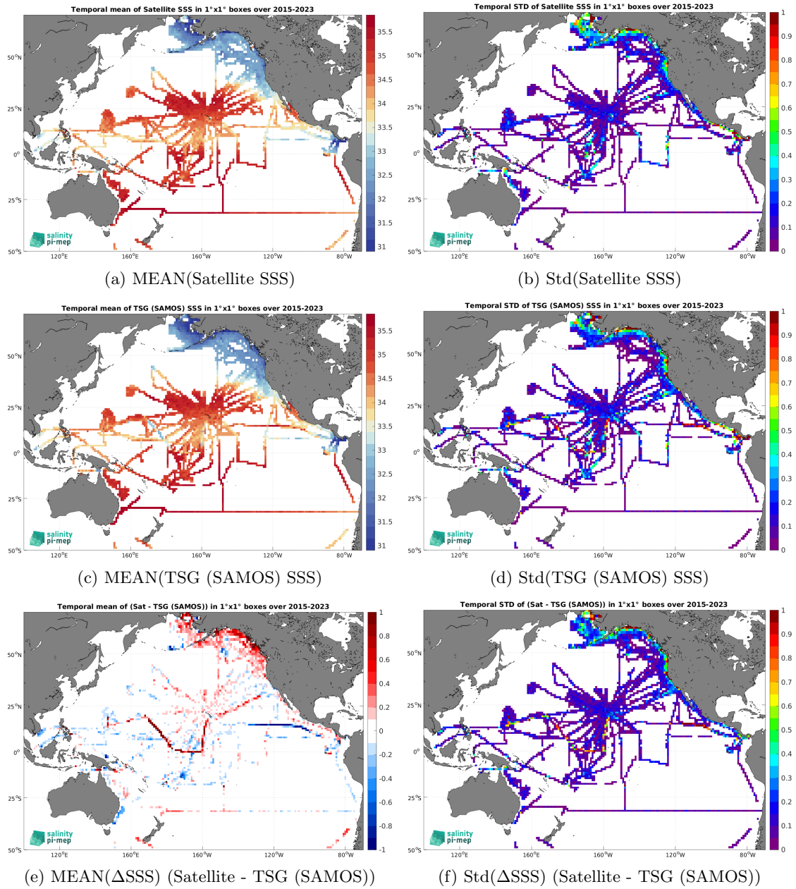
Figure 7: Temporal mean (left) and Std (right) of SSS from SMAP SSS L3 v5.3 - Monthly (RSS) (top), TSG (SAMOS) (middle), and of \Delta SSS (Satellite - TSG (SAMOS)). Only match-up pairs are used to generate these maps.
