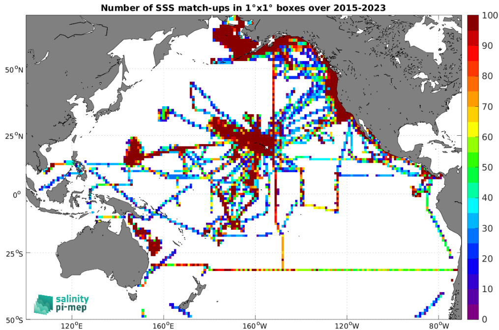
Figure 5: Number of SSS match-ups between TSG (SAMOS) SSS and the SMAP SSS L3 v5.3 - Monthly (RSS) SSS product for the Pacific Ocean Pi-MEP region over 1^\circ \times 1^\circ boxes and for the full satellite product period.
