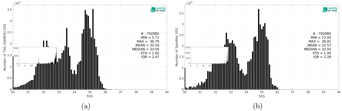
Figure 3: Histograms of SSS from TSG (SAMOS) (a) and SMAP SSS L3 v5.3 - Monthly (RSS) (b) considering all match-up pairs per bins of 0.1 over the Pacific Ocean Pi-MEP region and for the full satellite product period.
