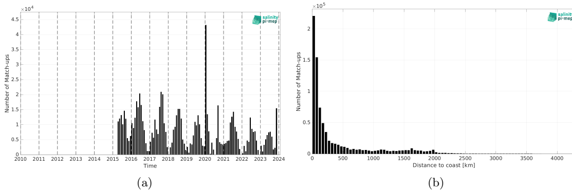
Figure 2: Number of match-ups between TSG (SAMOS) and SMAP SSS L3 v5.3 - Monthly (RSS) SSS as a function of time (a) and as function of the distance to coast (b) over the Pacific Ocean Pi-MEP region and for the full satellite product period.
