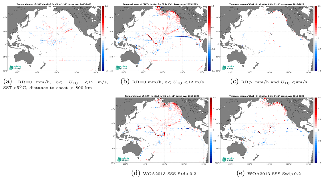
Figure 14: Temporal mean gridded over spatial boxes of size 1^\circ \times 1^\circ of \Delta\text{SSS} (SMAP SSS L3 v5.3 - Monthly (RSS) - TSG (SAMOS)) for 5 different subdatasets corresponding to:RR=0 mm/h, 3 < U_{10} < 12 m/s, SST >5^\circ\text{C} , distance to coast > 800 km (a), RR=0 mm/h, 3 < U_{10} < 12 m/s (b), RR >1 mm/h and U_{10} < 4 m/s (c), WOA2013 SSS Std <0.2 (d), WOA2013 SSS Std >0.2 (e).
