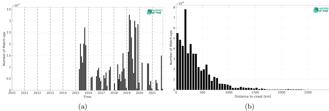
Figure 2: Number of match-ups between TSG (GOSUD-Research-vessel) and SMAP SSS L3 v5.3 - Monthly (RSS) SSS as a function of time (a) and as function of the distance to coast (b) over the Pacific Ocean Pi-MEP region and for the full satellite product period.
