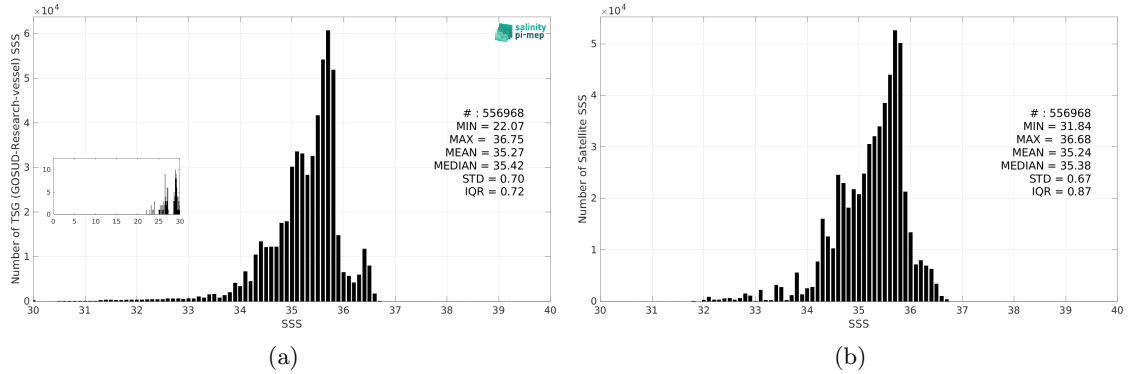
Figure 3: Histograms of SSS from TSG (GOSUD-Research-vessel) (a) and SMAP SSS L3 v5.3 - Monthly (RSS) (b) considering all match-up pairs per bins of 0.1 over the Pacific Ocean Pi-MEP region and for the full satellite product period.
