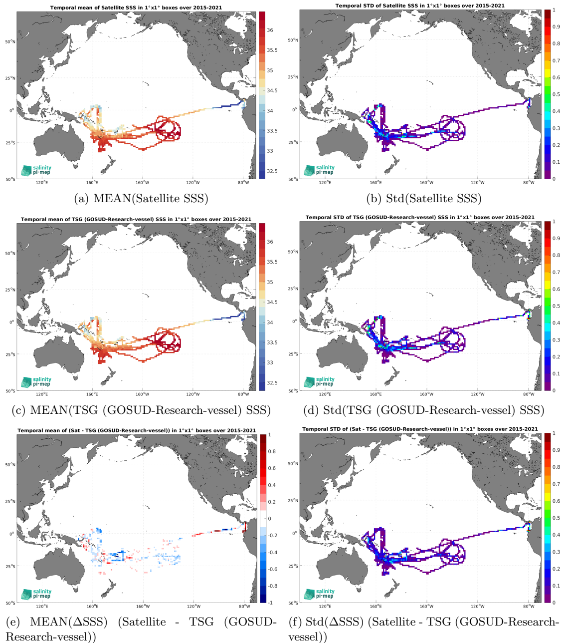
Figure 7: Temporal mean (left) and Std (right) of SSS from SMAP SSS L3 v5.3 - Monthly (RSS) (top), TSG (GOSUD-Research-vessel) (middle), and of \Delta SSS (Satellite - TSG (GOSUD-Research-vessel)). Only match-up pairs are used to generate these maps.
