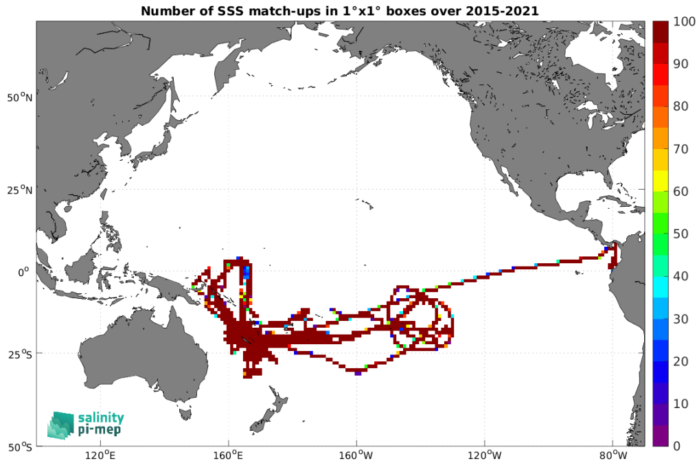
Figure 5: Number of SSS match-ups between TSG (GOSUD-Research-vessel) SSS and the SMAP SSS L3 v5.3 - Monthly (RSS) SSS product for the Pacific Ocean Pi-MEP region over 1^\circ \times 1^\circ boxes and for the full satellite product period.
