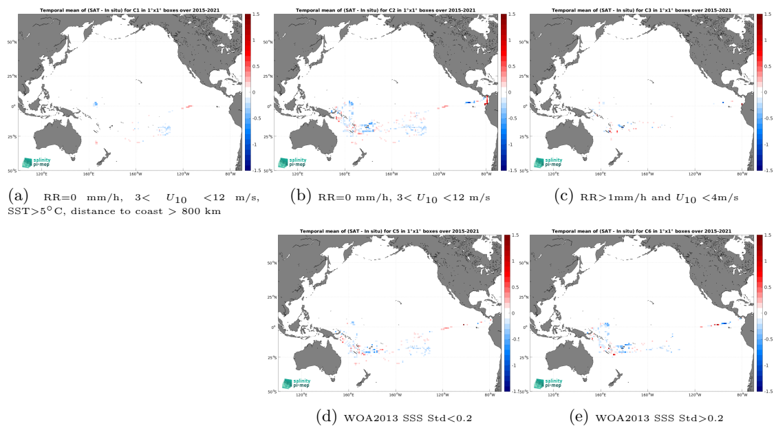
Figure 14: Temporal mean gridded over spatial boxes of size 1^\circ \times 1^\circ of \Delta SSS (SMAP SSS L3 v5.3 - Monthly (RSS) - TSG (GOSUD-Research-vessel)) for 5 different subdatasets corresponding to: RR=0 mm/h, 3 < U_{10} < 12 m/s, SST > 5^\circ\text{C} , distance to coast > 800 km (a), RR=0 mm/h, 3 < U_{10} < 12 m/s (b), RR > 1 mm/h and U_{10} < 4 m/s (c), WOA2013 SSS Std < 0.2 (d), WOA2013 SSS Std > 0.2 (e).
