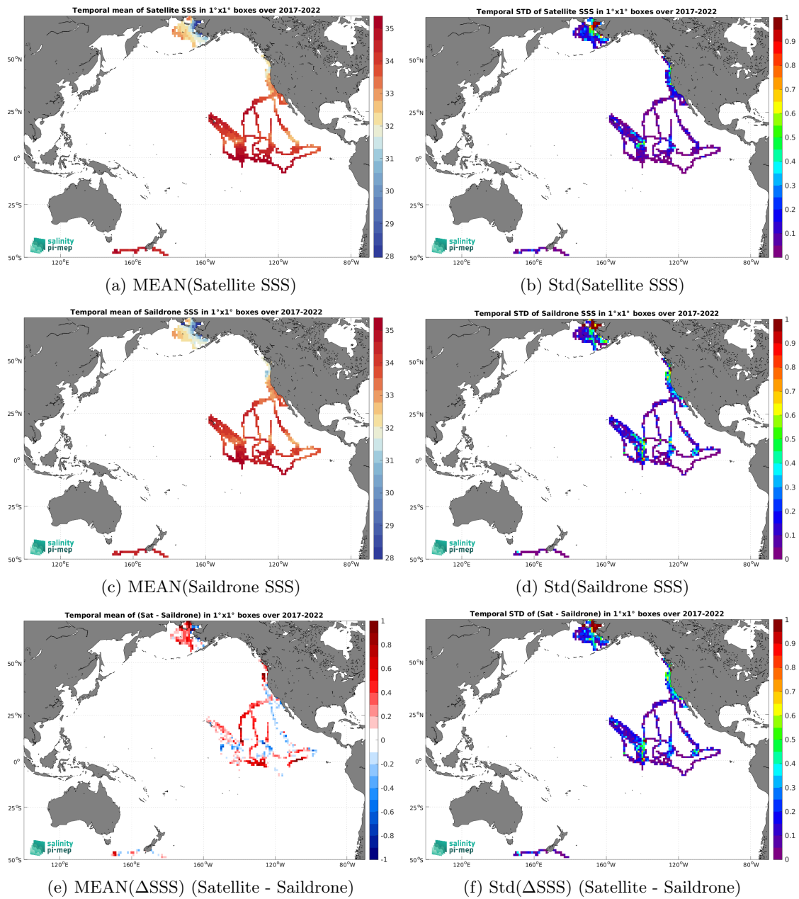
Figure 7: Temporal mean (left) and Std (right) of SSS from SMAP SSS L3 v5.3 - Monthly (RSS) (top), Saildrone (middle), and of \Delta SSS (Satellite - Saildrone). Only match-up pairs are used to generate these maps.
