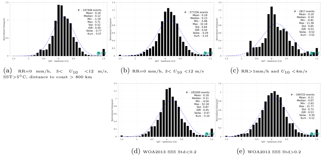
Figure 15: Normalized histogram of \Delta\text{SSS} (SMAP SSS L3 v5.3 - Monthly (RSS) - Saildrone) for 5 different subdatasets corresponding to: RR=0 mm/h, 3 < U_{10} < 12 m/s, SST>5°C, distance to coast > 800 km (a), RR=0 mm/h, 3 < U_{10} < 12 m/s (b), RR>1mm/h and U_{10} < 4 m/s (c), WOA2013 SSS Std<0.2 (d), WOA2013 SSS Std>0.2 (e).
