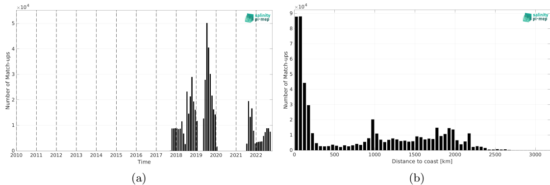
Figure 2: Number of match-ups between Saildrone and SMAP SSS L3 v5.3 - Monthly (RSS) SSS as a function of time (a) and as function of the distance to coast (b) over the Pacific Ocean Pi-MEP region and for the full satellite product period.
