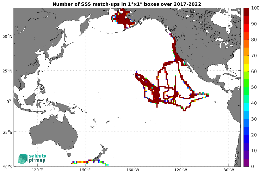
Figure 5: Number of SSS match-ups between Saildrone SSS and the SMAP SSS L3 v5.3 - Monthly (RSS) SSS product for the Pacific Ocean Pi-MEP region over 1^\circ \times 1^\circ boxes and for the full satellite product period.
