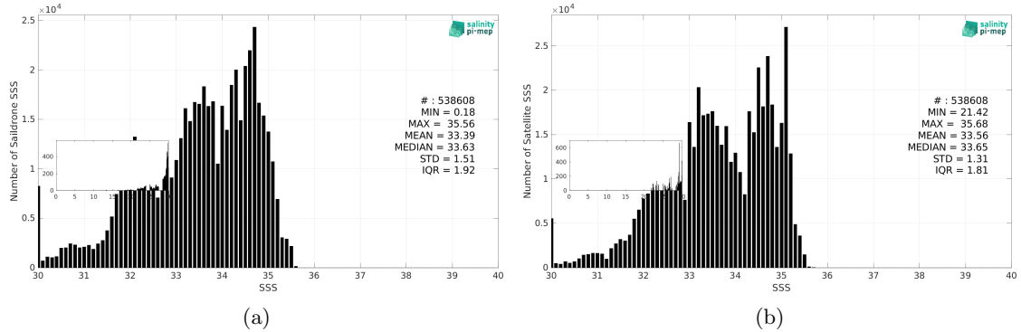
Figure 3: Histograms of SSS from Sairdrone (a) and SMAP SSS L3 v5.3 - Monthly (RSS) (b) considering all match-up pairs per bins of 0.1 over the Pacific Ocean Pi-MEP region and for the full satellite product period.
