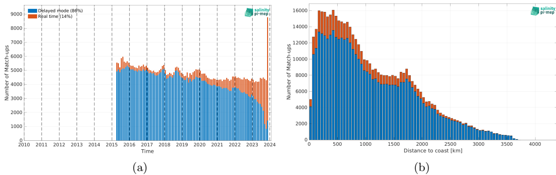
Figure 2: Number of match-ups between Argo and SMAP SSS L3 v5.3 - Monthly (RSS) SSS as a function of time (a) and as function of the distance to coast (b) over the Pacific Ocean Pi-MEP region and for the full satellite product period.
