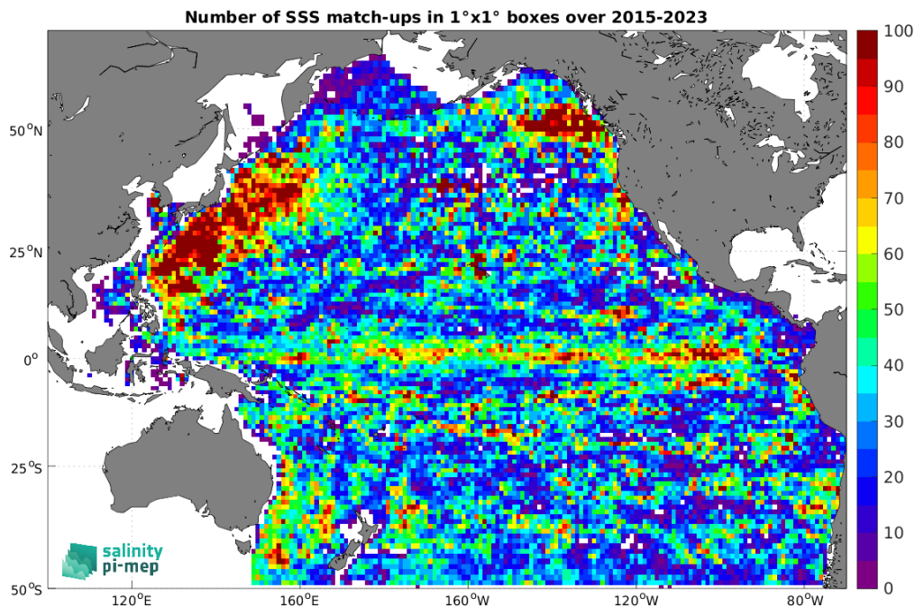
Figure 5: Number of SSS match-ups between Argo SSS and the SMAP SSS L3 v5.3 - Monthly (RSS) SSS product for the Pacific Ocean Pi-MEP region over 1^{\circ} \times 1^{\circ} boxes and for the full satellite product period.
