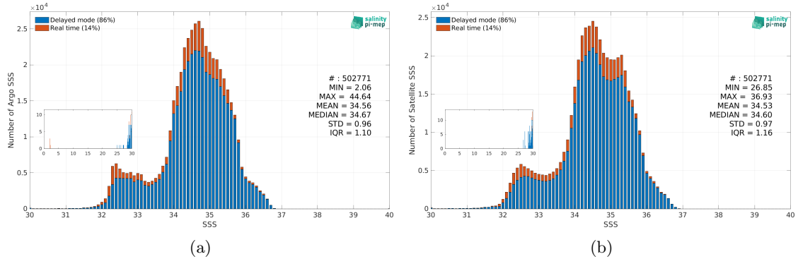
Figure 3: Histograms of SSS from Argo (a) and SMAP SSS L3 v5.3 - Monthly (RSS) (b) considering all match-up pairs per bins of 0.1 over the Pacific Ocean Pi-MEP region and for the full satellite product period.
