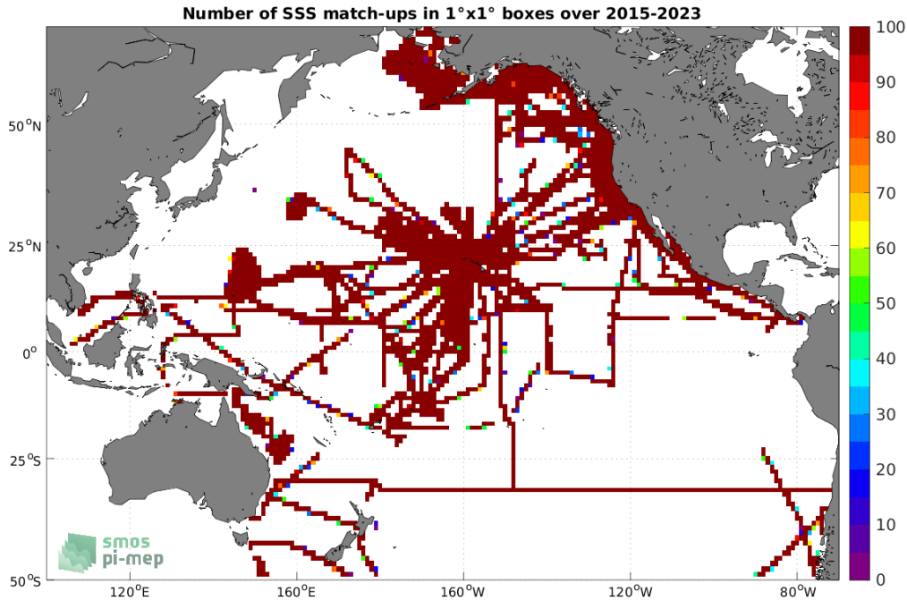
Figure 4: Number of SSS match-ups between TSG (SAMOS) SSS and the SMAP SSS L3 v5 - 8-Day running (RSS) SSS product for the Pacific Ocean Pi-MEP region over 1°x1° boxes and for the full satellite product period.
