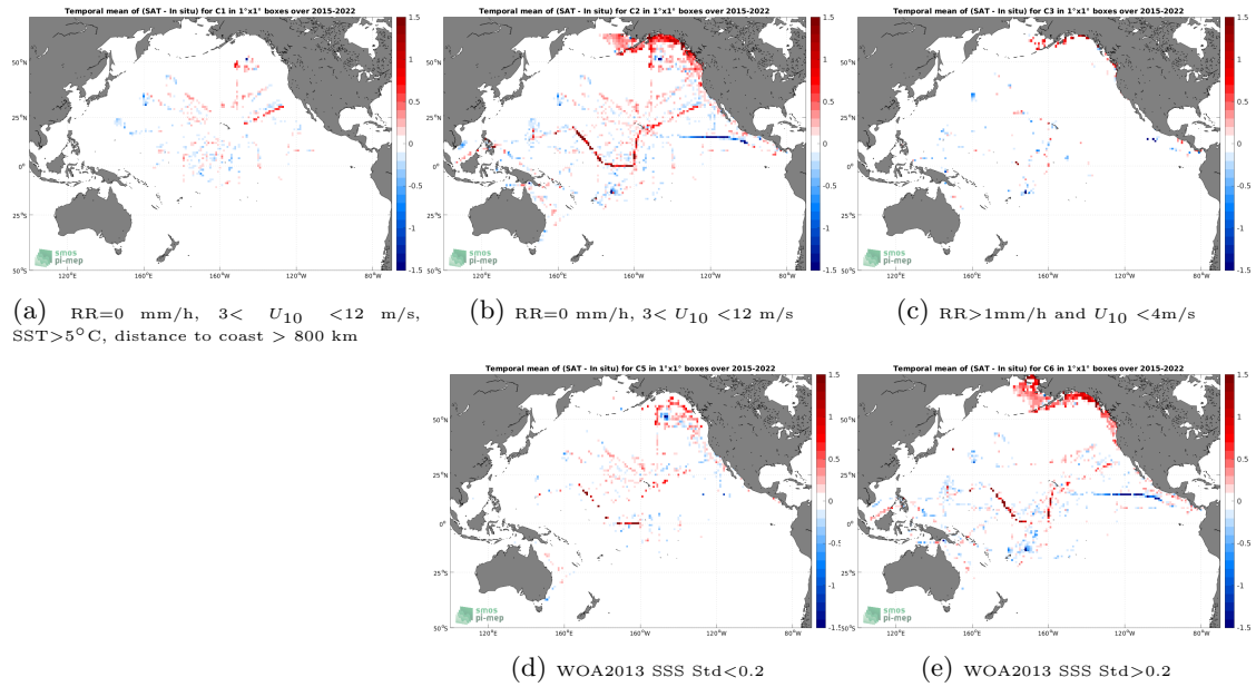
Figure 12: Temporal mean gridded over spatial boxes of size 1^\circ \times 1^\circ of \Delta\text{SSS} (SMAP SSS L3 v5 - 8-Day running (RSS) - TSG (SAMOS)) for 5 different subdatasets corresponding to:RR=0 mm/h, 3 < U_{10} < 12 m/s, SST >5^\circ\text{C} , distance to coast > 800 km (a), RR=0 mm/h, 3 < U_{10} < 12 m/s (b), RR >1 mm/h and U_{10} < 4 m/s (c), WOA2013 SSS Std <0.2 (d), WOA2013 SSS Std >0.2 (e).
