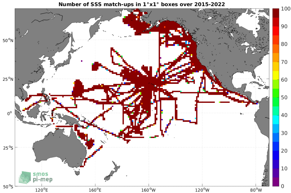
Figure 4: Number of SSS match-ups between TSG (SAMOS) SSS and the SMAP SSS L3 v5 - 8-Day running (RSS) SSS product for the Pacific Ocean Pi-MEP region over 1^\circ \times 1^\circ boxes and for the full satellite product period.
