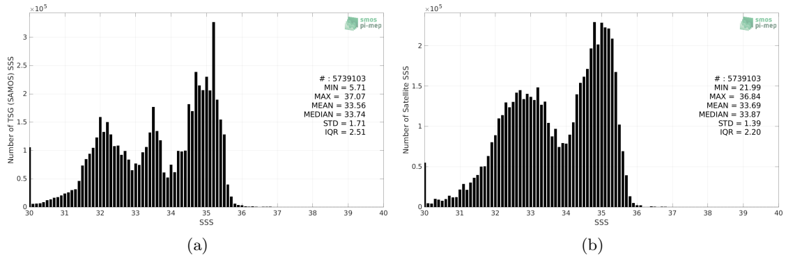
Figure 2: Histograms of SSS from TSG (SAMOS) (a) and SMAP SSS L3 v5 - 8-Day running (RSS) (b) considering all match-up pairs per bins of 0.1 over the Pacific Ocean Pi-MEP region and for the full satellite product period.
