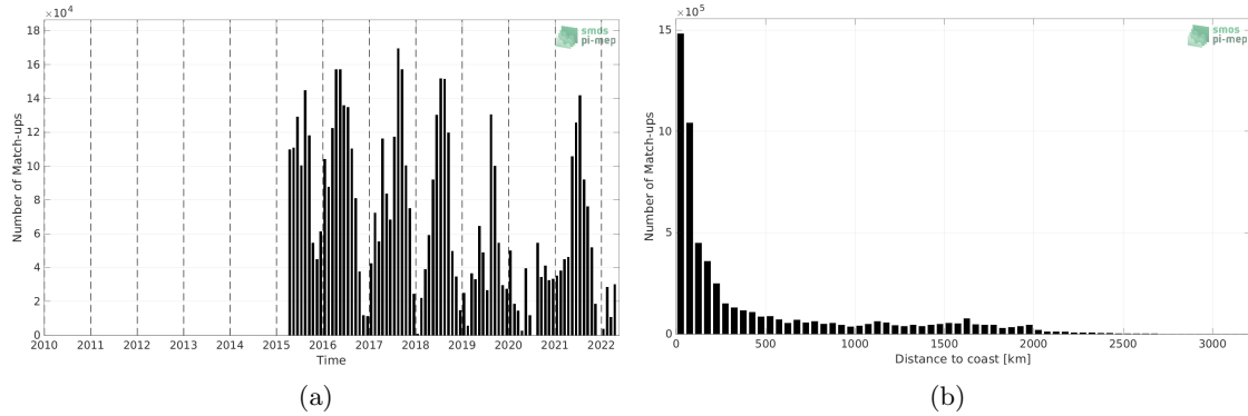
Figure 1: Number of match-ups between TSG (SAMOS) and SMAP SSS L3 v5 - 8-Day running (RSS) SSS as a function of time (a) and as function of the distance to coast (b) over the Pacific Ocean Pi-MEP region and for the full satellite product period.
