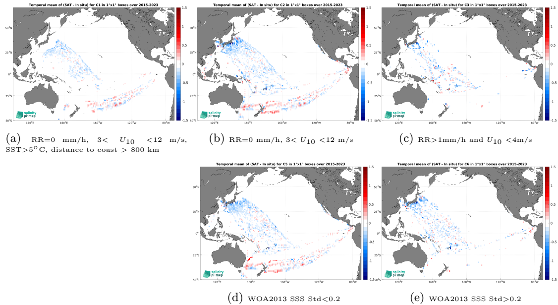
Figure 12: Temporal mean gridded over spatial boxes of size 1^\circ \times 1^\circ of \Delta\text{SSS} (SMAP SSS L3 v5 - 8-Day running (RSS) - TSG (LEGOS-DM)) for 5 different subdatasets corresponding to:RR=0 mm/h, 3 < U_{10} < 12 m/s, SST >5^\circ\text{C} , distance to coast > 800 km (a), RR=0 mm/h, 3 < U_{10} < 12 m/s (b), RR >1 mm/h and U_{10} < 4 m/s (c), WOA2013 SSS Std <0.2 (d), WOA2013 SSS Std >0.2 (e).
