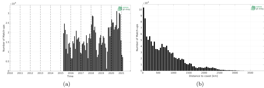
Figure 1: Number of match-ups between TSG (LEGOS-DM) and SMAP SSS L3 v5 - 8-Day running (RSS) SSS as a function of time (a) and as function of the distance to coast (b) over the Pacific Ocean Pi-MEP region and for the full satellite product period.
