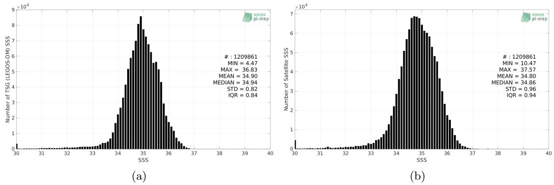
Figure 2: Histograms of SSS from TSG (LEGOS-DM) (a) and SMAP SSS L3 v5 - 8-Day running (RSS) (b) considering all match-up pairs per bins of 0.1 over the Pacific Ocean Pi-MEP region and for the full satellite product period.
