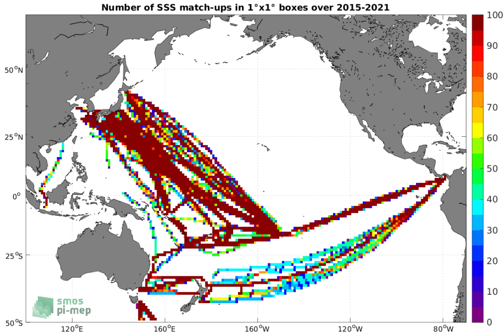
Figure 4: Number of SSS match-ups between TSG (LEGOS-DM) SSS and the SMAP SSS L3 v5 - 8-Day running (RSS) SSS product for the Pacific Ocean Pi-MEP region over 1^\circ \times 1^\circ boxes and for the full satellite product period.
