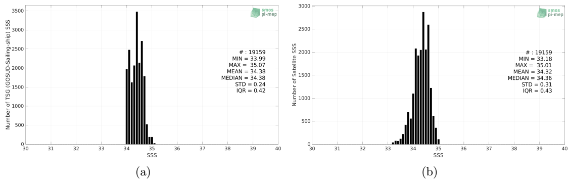
Figure 2: Histograms of SSS from TSG (GOSUD-Sailing-ship) (a) and SMAP SSS L3 v5 - 8-Day running (RSS) (b) considering all match-up pairs per bins of 0.1 over the Pacific Ocean Pi-MEP region and for the full satellite product period.
