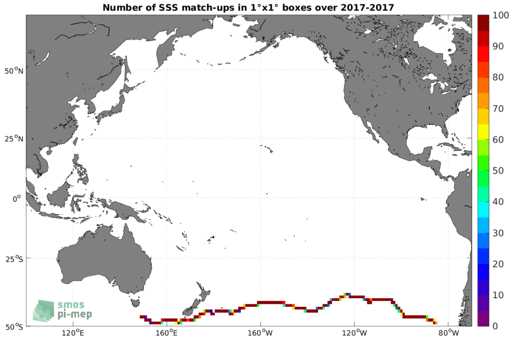
Figure 4: Number of SSS match-ups between TSG (GOSUD-Sailing-ship) SSS and the SMAP SSS L3 v5 - 8-Day running (RSS) SSS product for the Pacific Ocean Pi-MEP region over 1^\circ \times 1^\circ boxes and for the full satellite product period.
