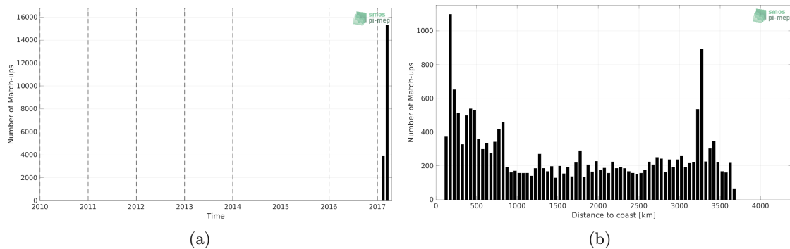
Figure 1: Number of match-ups between TSG (GOSUD-Sailing-ship) and SMAP SSS L3 v5 - 8-Day running (RSS) SSS as a function of time (a) and as function of the distance to coast (b) over the Pacific Ocean Pi-MEP region and for the full satellite product period.
