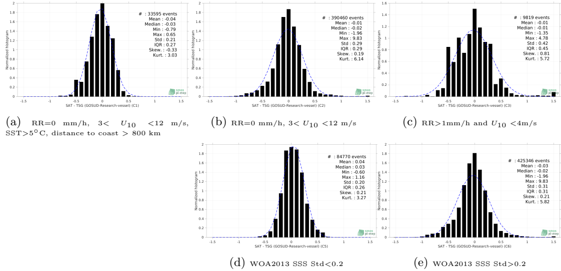
Figure 13: Normalized histogram of \Delta SSS (SMAP SSS L3 v5 - 8-Day running (RSS) - TSG (GOSUD-Research-vessel)) for 5 different subdatasets corresponding to: RR=0 mm/h, 3 < U_{10} < 12 m/s, SST > 5°C, distance to coast > 800 km (a), RR=0 mm/h, 3 < U_{10} < 12 m/s (b), RR > 1mm/h and U_{10} < 4 m/s (c), WOA2013 SSS Std < 0.2 (d), WOA2013 SSS Std > 0.2 (e).
