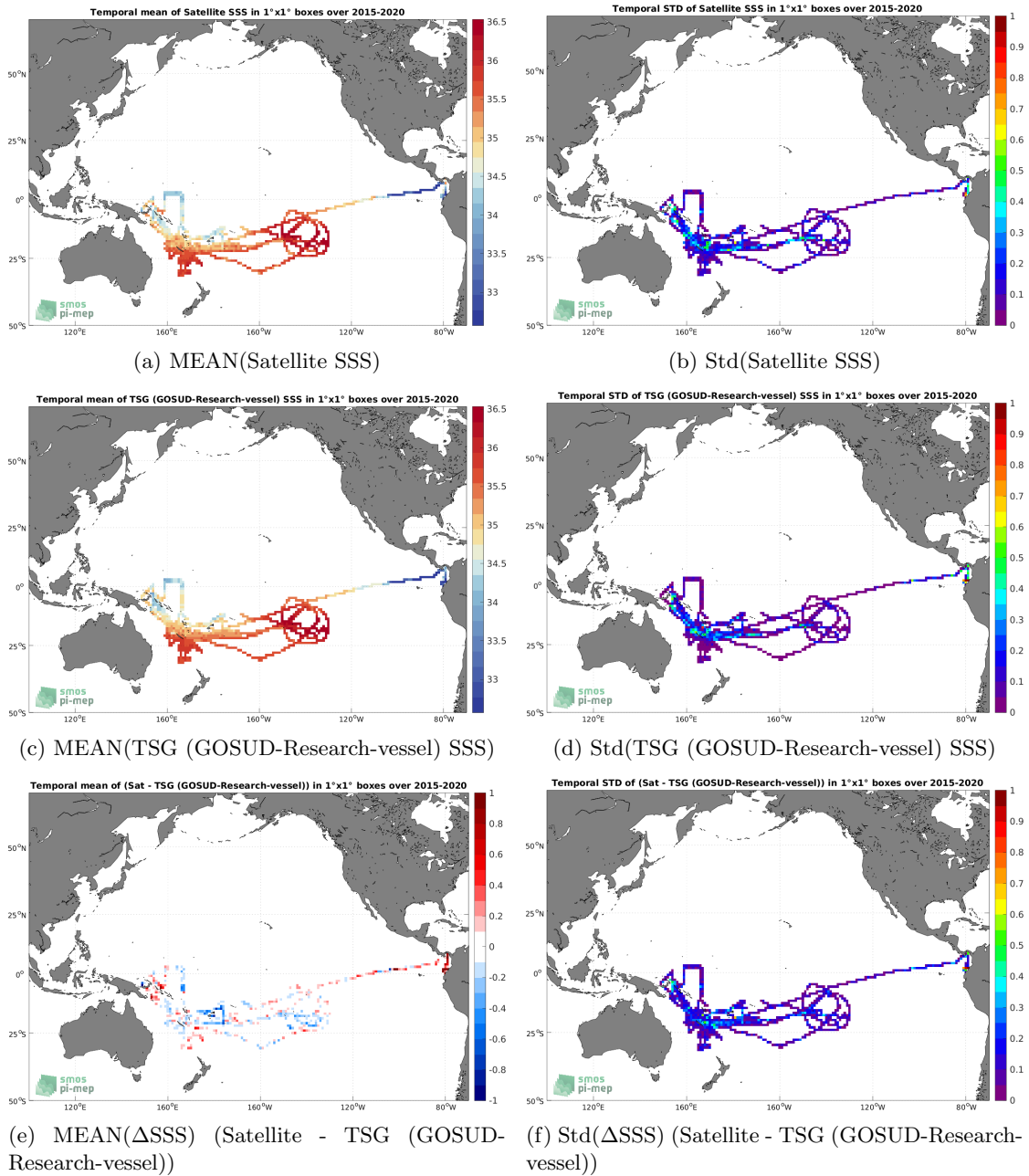
Figure 6: Temporal mean (left) and Std (right) of SSS from SMAP SSS L3 v5 - 8-Day running (RSS) (top), TSG (GOSUD-Research-vessel) (middle), and of \Delta SSS (Satellite - TSG (GOSUD-Research-vessel)). Only match-up pairs are used to generate these maps.
