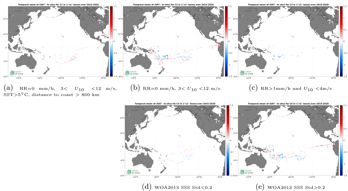
Figure 12: Temporal mean gridded over spatial boxes of size 1^\circ \times 1^\circ of \Delta SSS (SMAP SSS L3 v5 - 8-Day running (RSS) - TSG (GOSUD-Research-vessel)) for 5 different subdatasets corresponding to:RR=0 mm/h, 3 < U_{10} < 12 m/s, SST > 5^\circ\text{C} , distance to coast > 800 km (a), RR=0 mm/h, 3 < U_{10} < 12 m/s (b), RR > 1 mm/h and U_{10} < 4 m/s (c), WOA2013 SSS Std < 0.2 (d), WOA2013 SSS Std > 0.2 (e).
