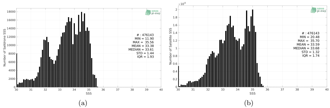
Figure 2: Histograms of SSS from Saildrone (a) and SMAP SSS L3 v5 - 8-Day running (RSS) (b) considering all match-up pairs per bins of 0.1 over the Pacific Ocean Pi-MEP region and for the full satellite product period.
