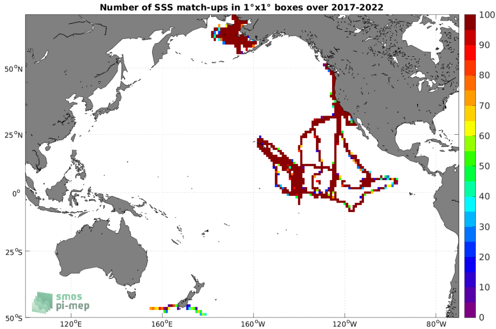
Figure 4: Number of SSS match-ups between Saildrone SSS and the SMAP SSS L3 v5 - 8-Day running (RSS) SSS product for the Pacific Ocean Pi-MEP region over 1^\circ \times 1^\circ boxes and for the full satellite product period.
