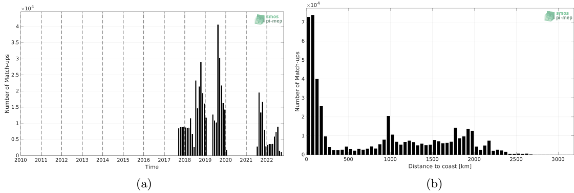
Figure 1: Number of match-ups between Saildrone and SMAP SSS L3 v5 - 8-Day running (RSS) SSS as a function of time (a) and as function of the distance to coast (b) over the Pacific Ocean Pi-MEP region and for the full satellite product period.
