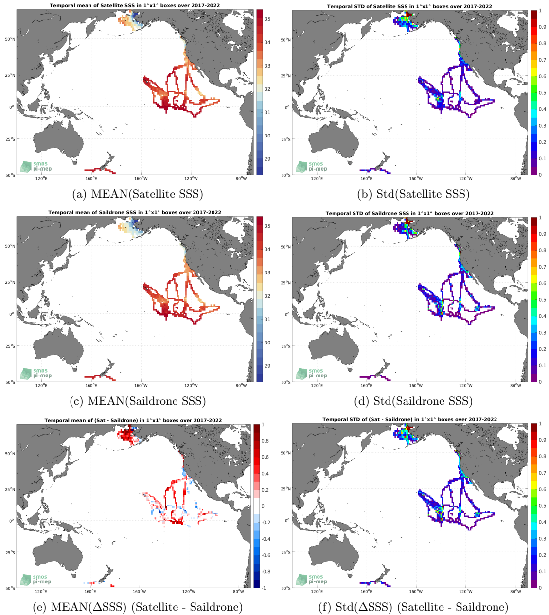
Figure 6: Temporal mean (left) and Std (right) of SSS from SMAP SSS L3 v5 - 8-Day running (RSS) (top), Saildrone (middle), and of \Delta SSS (Satellite - Saildrone). Only match-up pairs are used to generate these maps.
