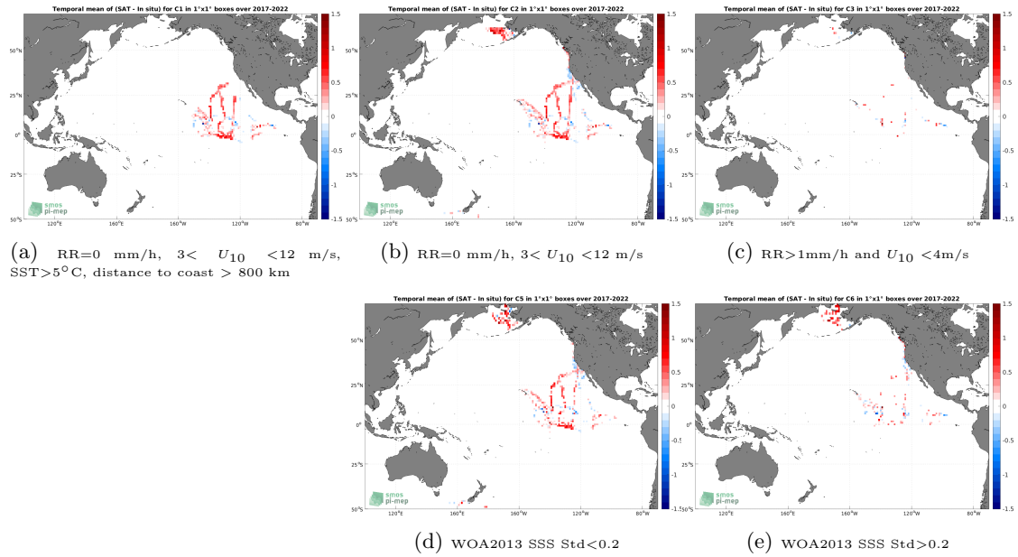
Figure 12: Temporal mean gridded over spatial boxes of size 1^\circ \times 1^\circ of \Delta SSS (SMAP SSS L3 v5 - 8-Day running (RSS) - Sairdrone) for 5 different subdatasets corresponding to:RR=0 mm/h, 3 < U_{10} < 12 m/s, SST >5^\circ C, distance to coast > 800 km (a), RR=0 mm/h, 3 < U_{10} < 12 m/s (b), RR >1 mm/h and U_{10} < 4 m/s (c), WOA2013 SSS Std <0.2 (d), WOA2013 SSS Std >0.2 (e).
