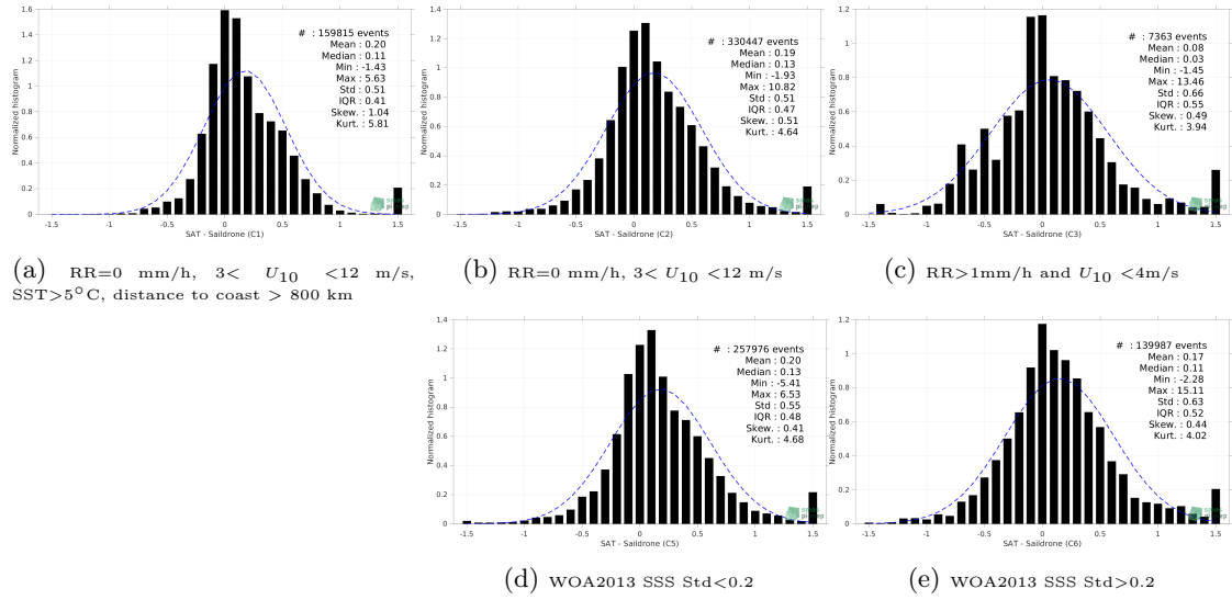
Figure 13: Normalized histogram of \Delta SSS (SMAP SSS L3 v5 - 8-Day running (RSS) - Sairdronne) for 5 different subdatasets corresponding to: RR=0 mm/h, 3 < U_{10} < 12 m/s, SST>5°C, distance to coast > 800 km (a), RR=0 mm/h, 3 < U_{10} < 12 m/s (b), RR>1mm/h and U_{10} < 4 m/s (c), WOA2013 SSS Std<0.2 (d), WOA2013 SSS Std>0.2 (e).
