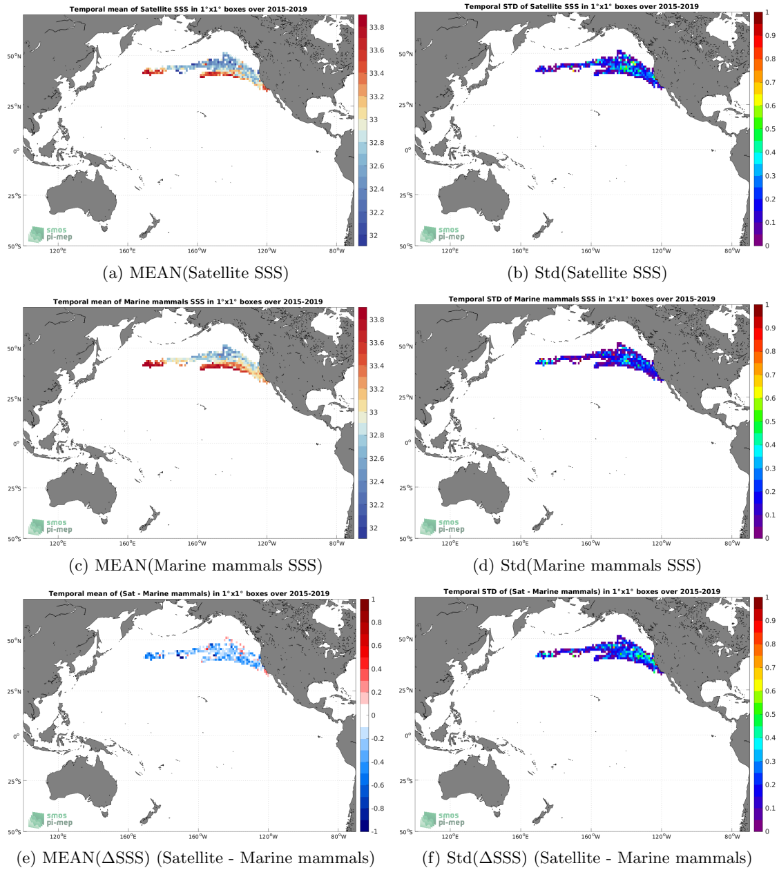
Figure 6: Temporal mean (left) and Std (right) of SSS from SMAP SSS L3 v5 - 8-Day running (RSS) (top), Marine mammals (middle), and of \Delta SSS (Satellite - Marine mammals). Only match-up pairs are used to generate these maps.
