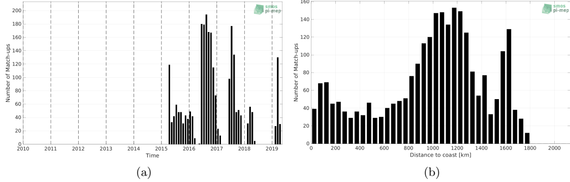
Figure 1: Number of match-ups between Marine mammals and SMAP SSS L3 v5 - 8-Day running (RSS) SSS as a function of time (a) and as function of the distance to coast (b) over the Pacific Ocean Pi-MEP region and for the full satellite product period.
