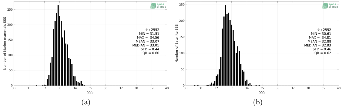
Figure 2: Histograms of SSS from Marine mammals (a) and SMAP SSS L3 v5 - 8-Day running (RSS) (b) considering all match-up pairs per bins of 0.1 over the Pacific Ocean Pi-MEP region and for the full satellite product period.
