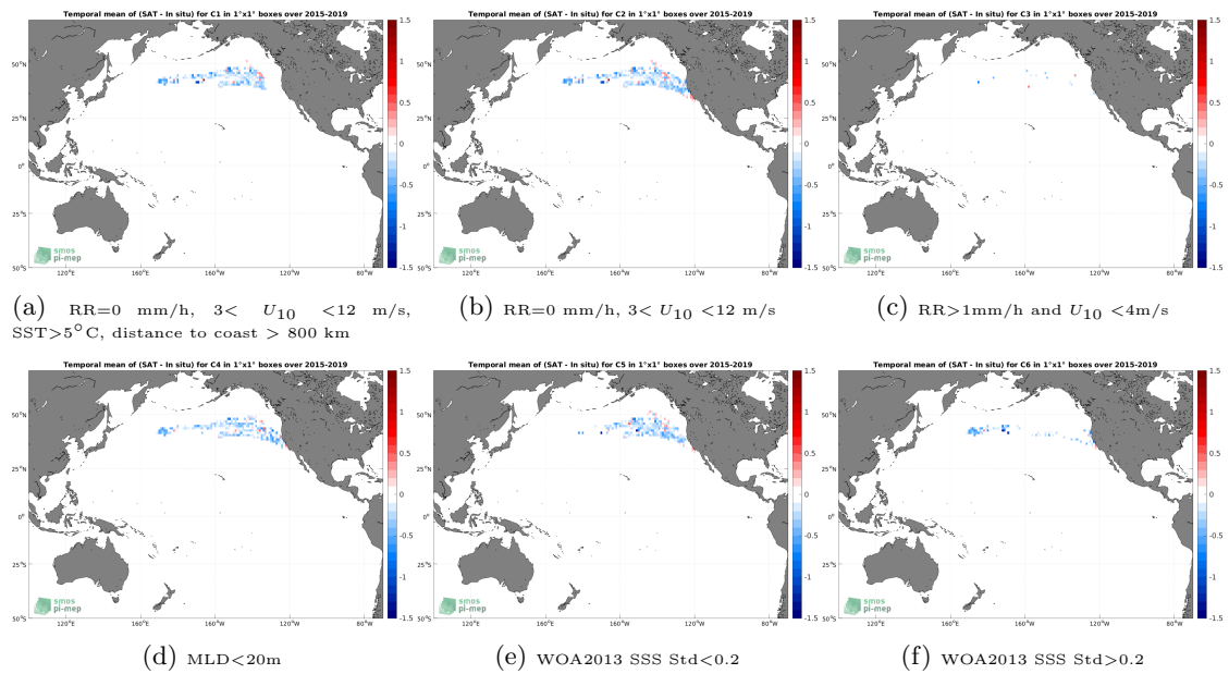
Figure 12: Temporal mean gridded over spatial boxes of size 1^\circ \times 1^\circ of \Delta SSS (SMAP SSS L3 v5 - 8-Day running (RSS) - Marine mammals) for 6 different subdatasets corresponding to:RR=0 mm/h, 3 < U_{10} < 12 m/s, SST > 5^\circ\text{C} , distance to coast > 800 km (a), RR=0 mm/h, 3 < U_{10} < 12 m/s (b), RR > 1 mm/h and U_{10} < 4 m/s (c),MLD < 20 m (d),WOA2013 SSS Std < 0.2 (e),WOA2013 SSS Std > 0.2 (f).
