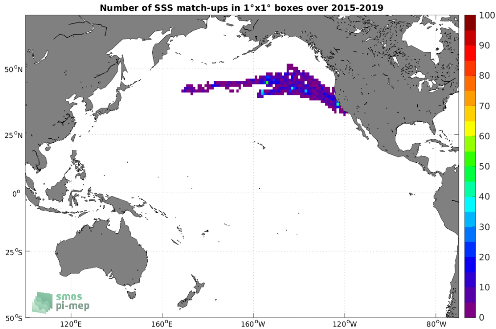
Figure 4: Number of SSS match-ups between Marine mammals SSS and the SMAP SSS L3 v5 - 8-Day running (RSS) SSS product for the Pacific Ocean Pi-MEP region over 1^\circ \times 1^\circ boxes and for the full satellite product period.
