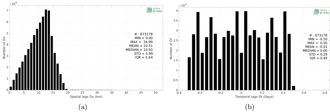
Figure 4: Histograms of the spatial (a) and temporal (b) lags between the location/time of the Surface drifters measurement and the date of the corresponding SMAP SSS L3 v5 - 8-Day running (RSS) SSS pixel.
