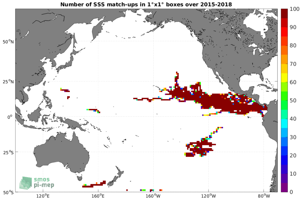
Figure 3: Number of SSS match-ups between Surface drifters SSS and the SMAP SSS L3 v5 - 8-Day running (RSS) SSS product for the Pacific Ocean Pi-MEP region over 1^\circ \times 1^\circ boxes and for the full satellite product period.
