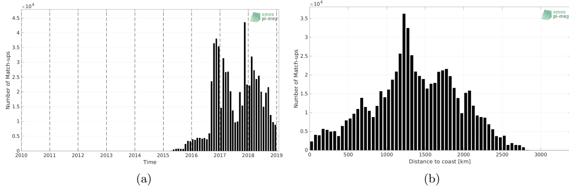
Figure 1: Number of match-ups between Surface drifters and SMAP SSS L3 v5 - 8-Day running (RSS) SSS as a function of time (a) and as function of the distance to coast (b) over the Pacific Ocean Pi-MEP region and for the full satellite product period.
