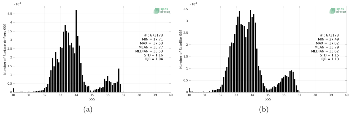
Figure 2: Histograms of SSS from Surface drifters (a) and SMAP SSS L3 v5 - 8-Day running (RSS) (b) considering all match-up pairs per bins of 0.1 over the Pacific Ocean Pi-MEP region and for the full satellite product period.
