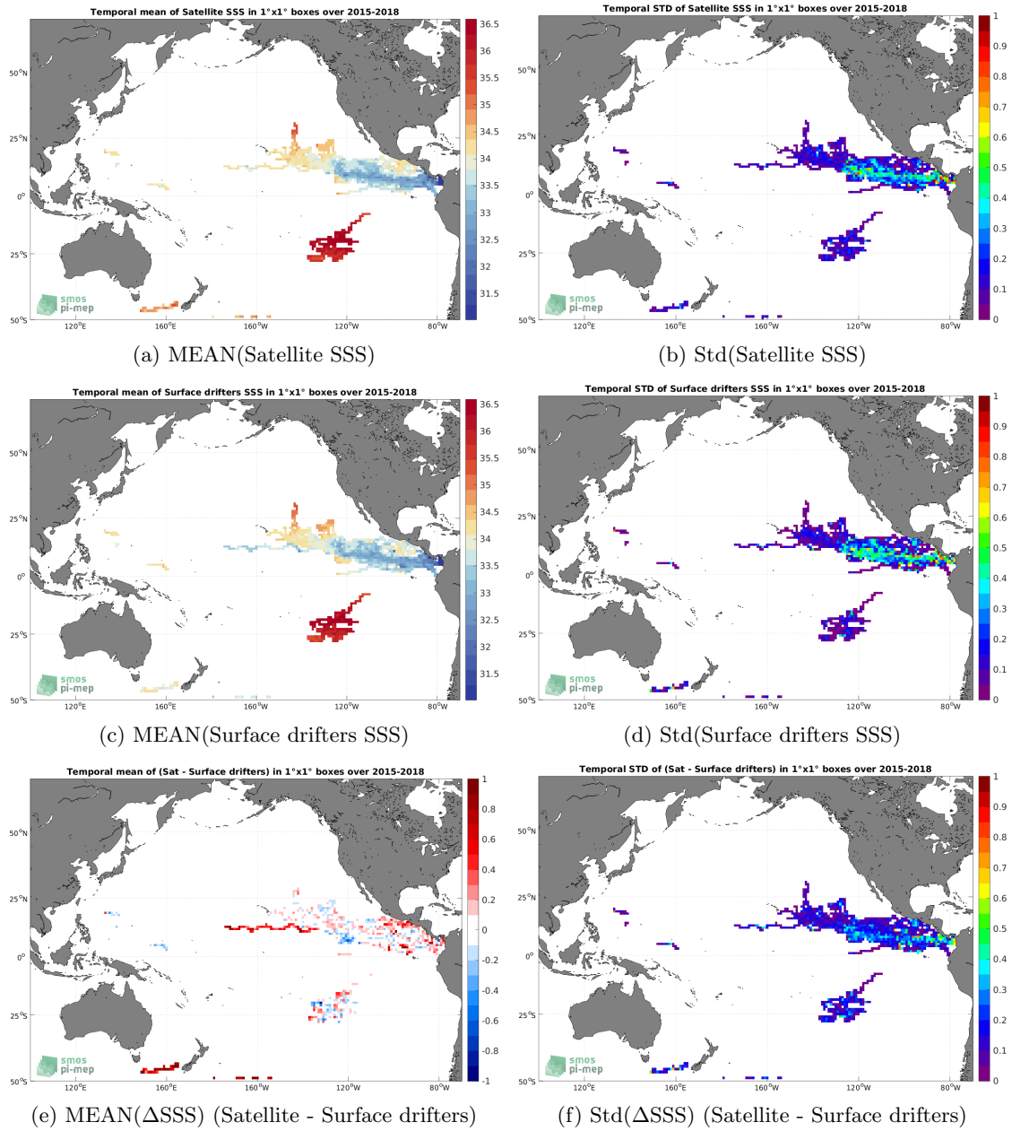
Figure 5: Temporal mean (left) and Std (right) of SSS from SMAP SSS L3 v5 - 8-Day running (RSS) (top), Surface drifters (middle), and of \Delta SSS (Satellite - Surface drifters). Only match-up pairs are used to generate these maps.
