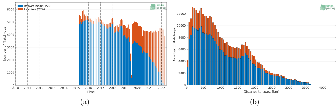
Figure 1: Number of match-ups between Argo and SMAP SSS L3 v5 - 8-Day running (RSS) SSS as a function of time (a) and as function of the distance to coast (b) over the Pacific Ocean Pi-MEP region and for the full satellite product period.
