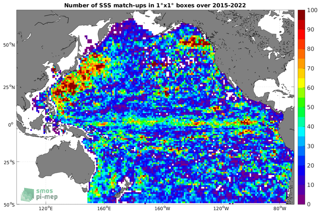
Figure 4: Number of SSS match-ups between Argo SSS and the SMAP SSS L3 v5 - 8-Day running (RSS) SSS product for the Pacific Ocean Pi-MEP region over 1^\circ \times 1^\circ boxes and for the full satellite product period.
