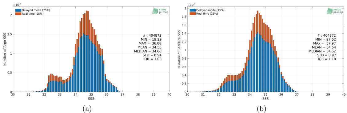
Figure 2: Histograms of SSS from Argo (a) and SMAP SSS L3 v5 - 8-Day running (RSS) (b) considering all match-up pairs per bins of 0.1 over the Pacific Ocean Pi-MEP region and for the full satellite product period.
