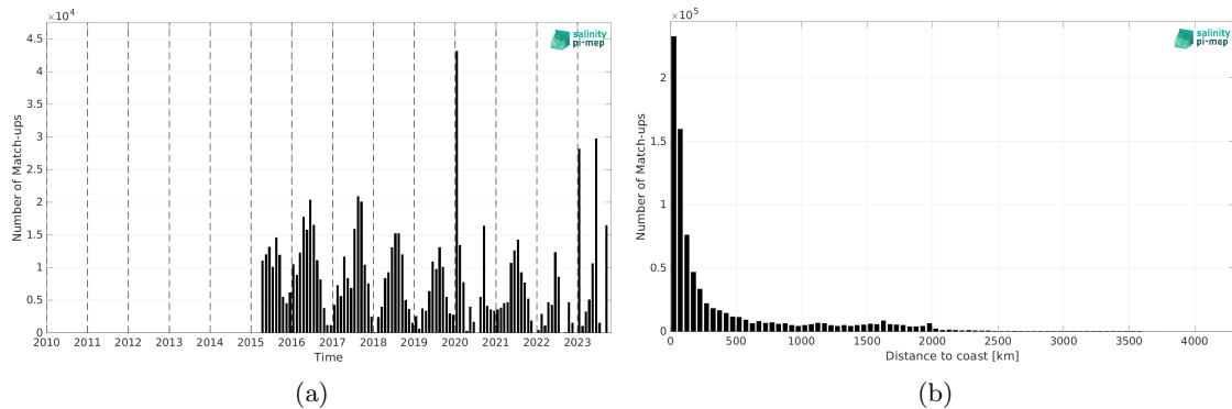
Figure 1: Number of match-ups between TSG (SAMOS) and SMAP SSS L3 v5 - Monthly (RSS) SSS as a function of time (a) and as function of the distance to coast (b) over the Pacific Ocean Pi-MEP region and for the full satellite product period.
