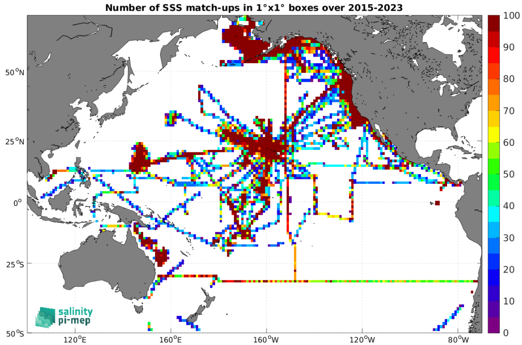
Figure 4: Number of SSS match-ups between TSG (SAMOS) SSS and the SMAP SSS L3 v5 - Monthly (RSS) SSS product for the Pacific Ocean Pi-MEP region over 1^\circ \times 1^\circ boxes and for the full satellite product period.
