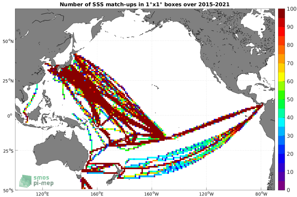
Figure 4: Number of SSS match-ups between TSG (LEGOS-DM) SSS and the SMAP SSS L3 v5 - Monthly (RSS) SSS product for the Pacific Ocean Pi-MEP region over 1^\circ \times 1^\circ boxes and for the full satellite product period.
