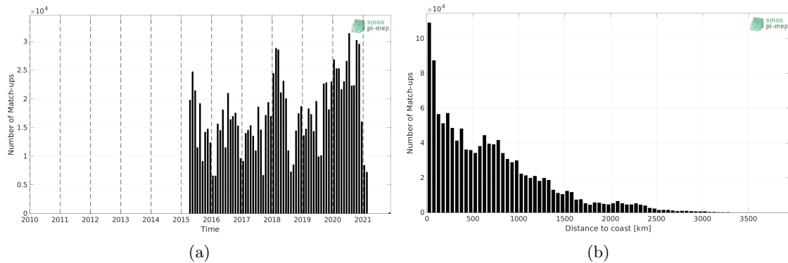
Figure 1: Number of match-ups between TSG (LEGOS-DM) and SMAP SSS L3 v5 - Monthly (RSS) SSS as a function of time (a) and as function of the distance to coast (b) over the Pacific Ocean Pi-MEP region and for the full satellite product period.
