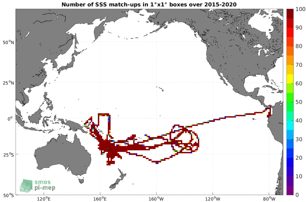
Figure 4: Number of SSS match-ups between TSG (GOSUD-Research-vessel) SSS and the SMAP SSS L3 v5 - Monthly (RSS) SSS product for the Pacific Ocean Pi-MEP region over 1^\circ \times 1^\circ boxes and for the full satellite product period.
