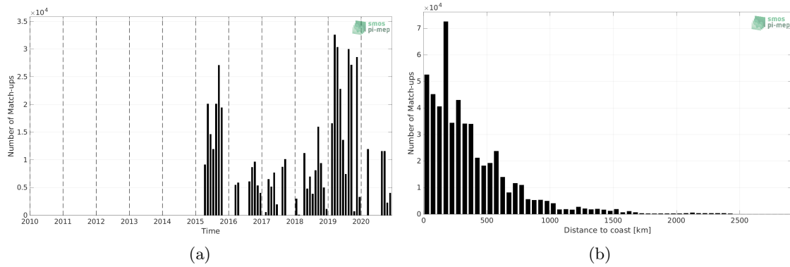
Figure 1: Number of match-ups between TSG (GOSUD-Research-vessel) and SMAP SSS L3 v5 - Monthly (RSS) SSS as a function of time (a) and as function of the distance to coast (b) over the Pacific Ocean Pi-MEP region and for the full satellite product period.
