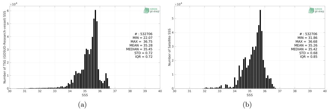
Figure 2: Histograms of SSS from TSG (GOSUD-Research-vessel) (a) and SMAP SSS L3 v5 - Monthly (RSS) (b) considering all match-up pairs per bins of 0.1 over the Pacific Ocean Pi-MEP region and for the full satellite product period.
