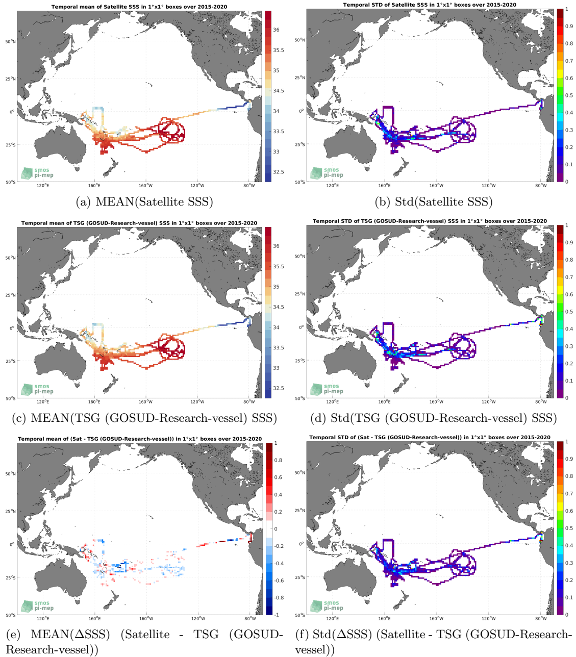
Figure 6: Temporal mean (left) and Std (right) of SSS from SMAP SSS L3 v5 - Monthly (RSS) (top), TSG (GOSUD-Research-vessel) (middle), and of \Delta SSS (Satellite - TSG (GOSUD-Research-vessel)). Only match-up pairs are used to generate these maps.
