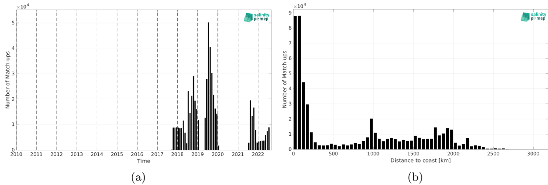
Figure 1: Number of match-ups between Sairdrone and SMAP SSS L3 v5 - Monthly (RSS) SSS as a function of time (a) and as function of the distance to coast (b) over the Pacific Ocean Pi-MEP region and for the full satellite product period.
