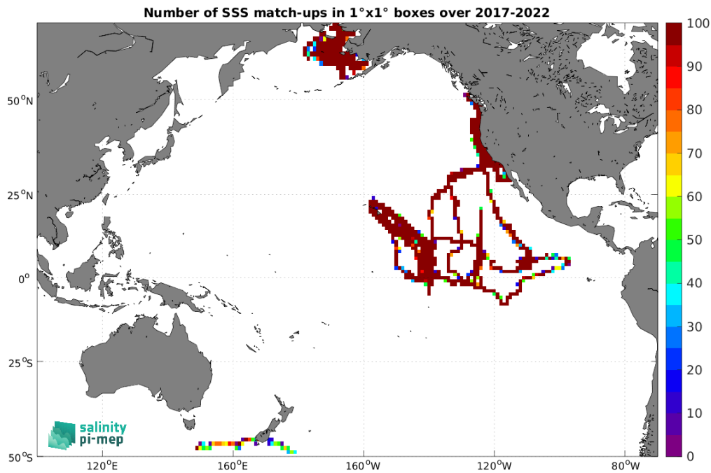
Figure 4: Number of SSS match-ups between Saildrone SSS and the SMAP SSS L3 v5 - Monthly (RSS) SSS product for the Pacific Ocean Pi-MEP region over 1^\circ \times 1^\circ boxes and for the full satellite product period.
