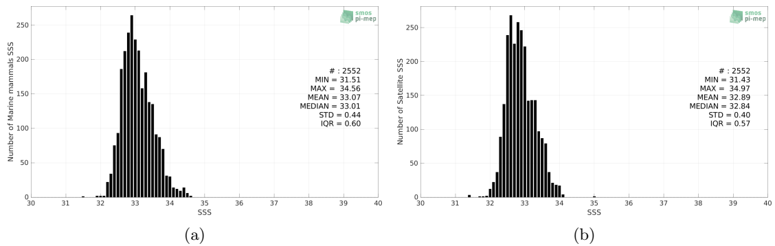
Figure 2: Histograms of SSS from Marine mammals (a) and SMAP SSS L3 v5 - Monthly (RSS) (b) considering all match-up pairs per bins of 0.1 over the Pacific Ocean Pi-MEP region and for the full satellite product period.
