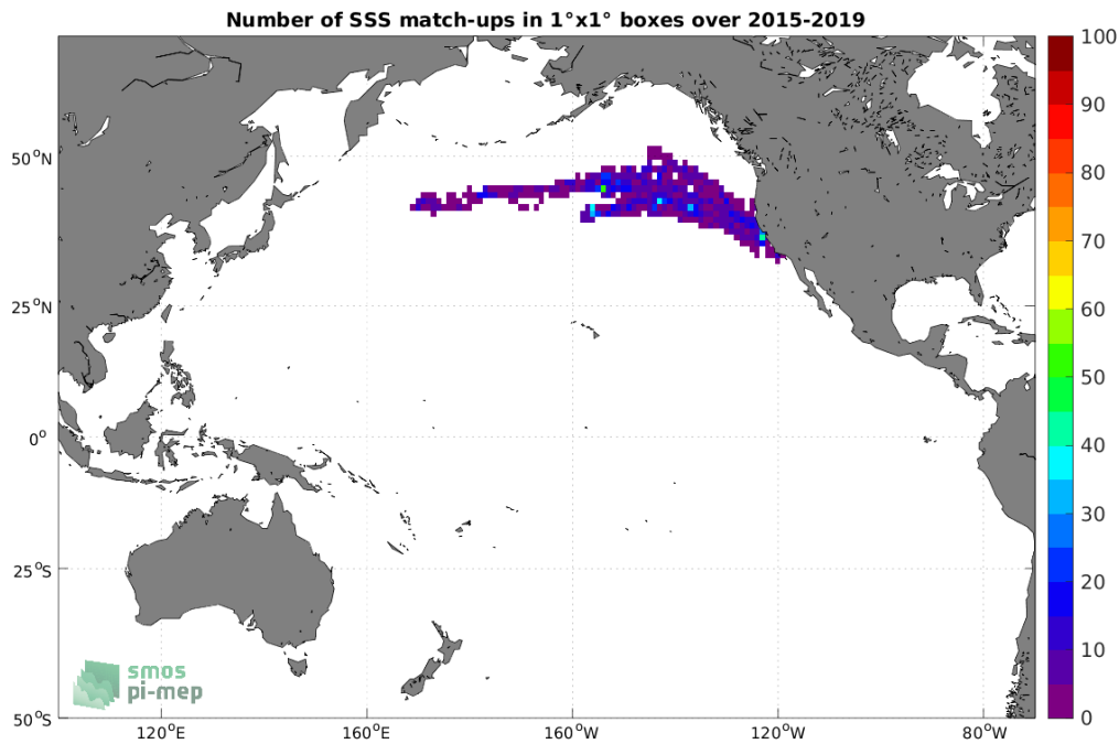
Figure 4: Number of SSS match-ups between Marine mammals SSS and the SMAP SSS L3 v5 - Monthly (RSS) SSS product for the Pacific Ocean Pi-MEP region over 1^\circ \times 1^\circ boxes and for the full satellite product period.
