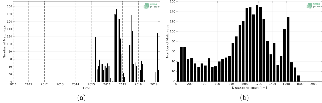
Figure 1: Number of match-ups between Marine mammals and SMAP SSS L3 v5 - Monthly (RSS) SSS as a function of time (a) and as function of the distance to coast (b) over the Pacific Ocean Pi-MEP region and for the full satellite product period.
