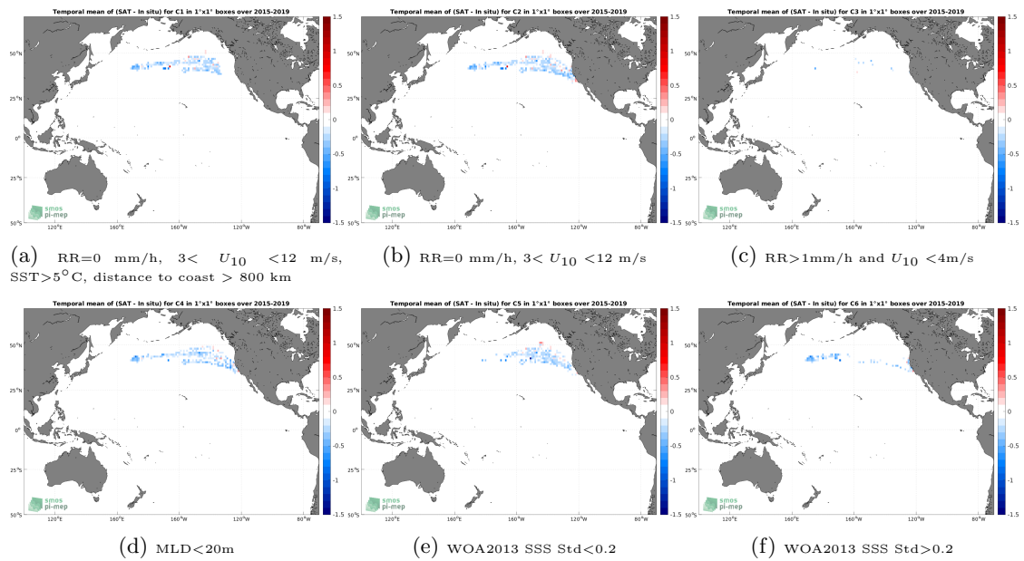
Figure 12: Temporal mean gridded over spatial boxes of size 1^\circ \times 1^\circ of \Delta SSS (SMAP SSS L3 v5 - Monthly (RSS) - Marine mammals) for 6 different subdatasets corresponding to:RR=0 mm/h, 3 < U_{10} < 12 m/s, SST >5^\circ C, distance to coast > 800 km (a), RR=0 mm/h, 3 < U_{10} < 12 m/s (b), RR >1 mm/h and U_{10} < 4 m/s (c),MLD <20 m (d),WOA2013 SSS Std <0.2 (e),WOA2013 SSS Std >0.2 (f).
