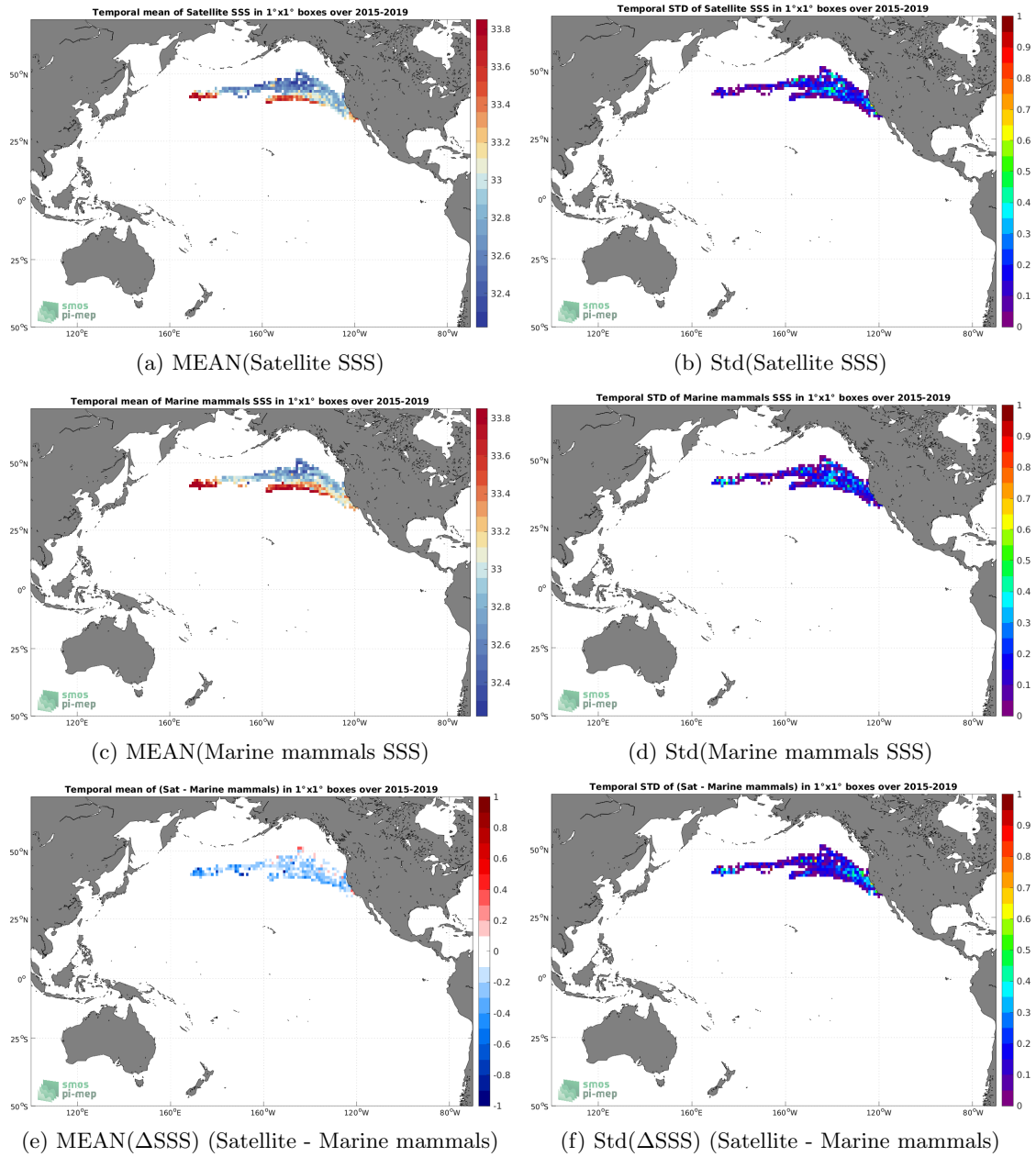
Figure 6: Temporal mean (left) and Std (right) of SSS from SMAP SSS L3 v5 - Monthly (RSS) (top), Marine mammals (middle), and of \Delta SSS (Satellite - Marine mammals). Only match-up pairs are used to generate these maps.
