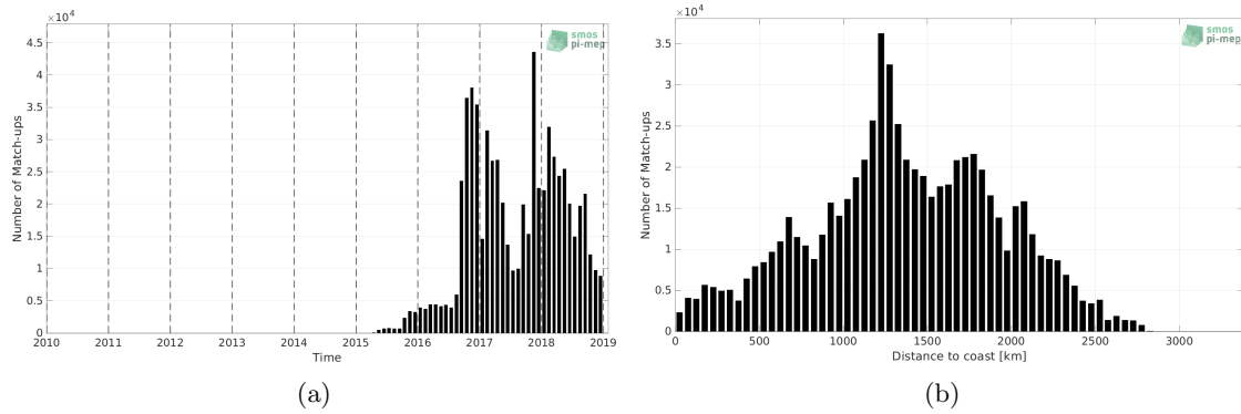
Figure 1: Number of match-ups between Surface drifters and SMAP SSS L3 v5 - Monthly (RSS) SSS as a function of time (a) and as function of the distance to coast (b) over the Pacific Ocean Pi-MEP region and for the full satellite product period.
