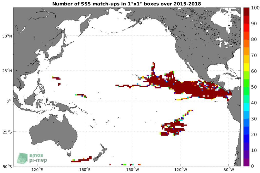
Figure 3: Number of SSS match-ups between Surface drifters SSS and the SMAP SSS L3 v5 - Monthly (RSS) SSS product for the Pacific Ocean Pi-MEP region over 1^\circ \times 1^\circ boxes and for the full satellite product period.
