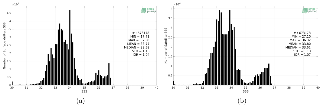
Figure 2: Histograms of SSS from Surface drifters (a) and SMAP SSS L3 v5 - Monthly (RSS) (b) considering all match-up pairs per bins of 0.1 over the Pacific Ocean Pi-MEP region and for the full satellite product period.
