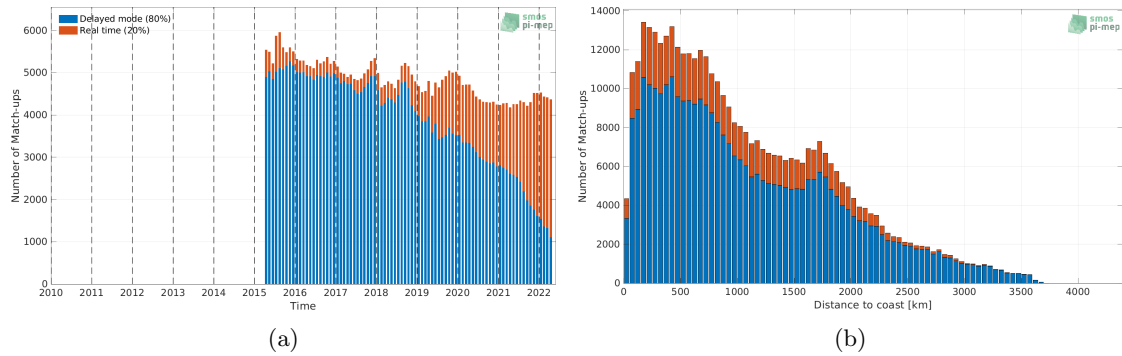
Figure 1: Number of match-ups between Argo and SMAP SSS L3 v5 - Monthly (RSS) SSS as a function of time (a) and as function of the distance to coast (b) over the Pacific Ocean Pi-MEP region and for the full satellite product period.
