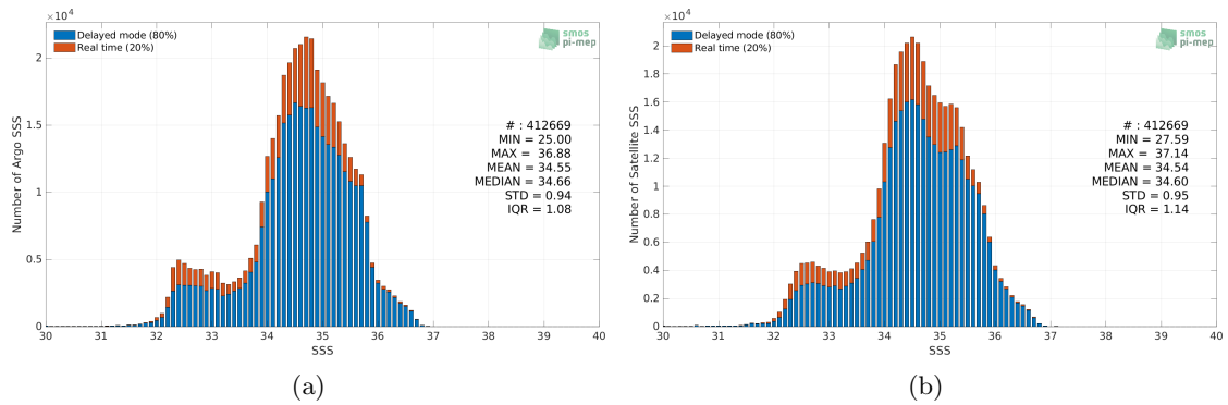
Figure 2: Histograms of SSS from Argo (a) and SMAP SSS L3 v5 - Monthly (RSS) (b) considering all match-up pairs per bins of 0.1 over the Pacific Ocean Pi-MEP region and for the full satellite product period.
