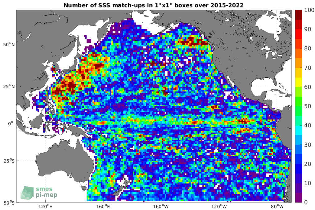
Figure 4: Number of SSS match-ups between Argo SSS and the SMAP SSS L3 v5 - Monthly (RSS) SSS product for the Pacific Ocean Pi-MEP region over 1^\circ \times 1^\circ boxes and for the full satellite product period.
