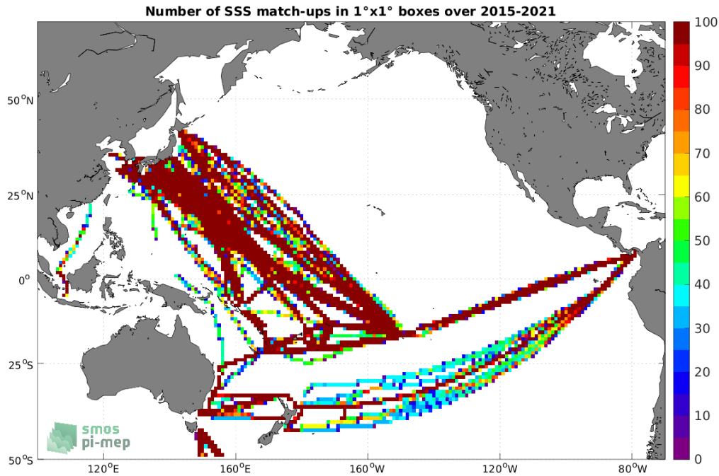
Figure 4: Number of SSS match-ups between TSG (LEGOS-DM) SSS and the SMAP SSS L3 v4 - 8-Day running (RSS) SSS product for the Pacific Ocean Pi-MEP region over 1^\circ \times 1^\circ boxes and for the full satellite product period.
