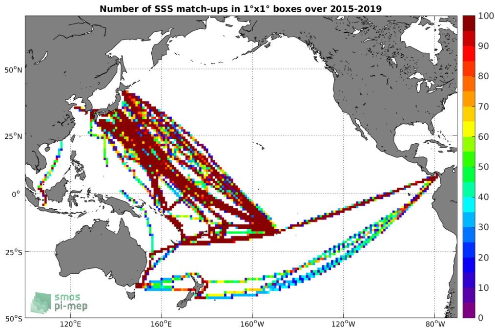
Figure 4: Number of SSS match-ups between TSG-LEGOS-DM SSS and the SMAP-L3-RSS-V4-8DAY-RUNNING SSS product for the Pacific Ocean Pi-MEP region over 1^\circ \times 1^\circ boxes and for the full satellite product period.
