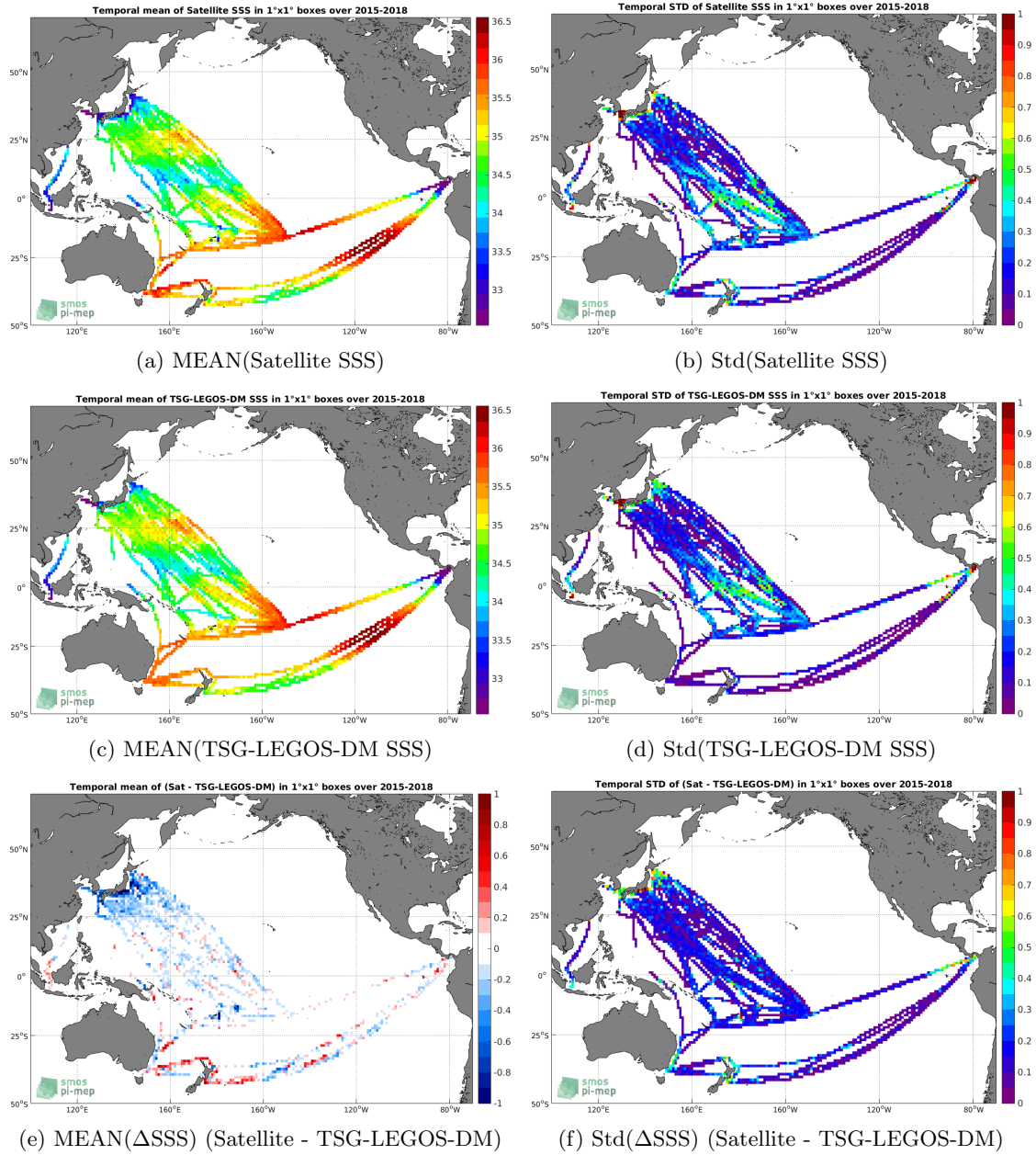
Figure 6: Temporal mean (left) and Std (right) of SSS from SMAP-L3-RSS-V4-8DAY-RUNNING (top), TSG-LEGOS-DM (middle), and of \Delta SSS (Satellite - TSG-LEGOS-DM). Only match-up pairs are used to generate these maps.
