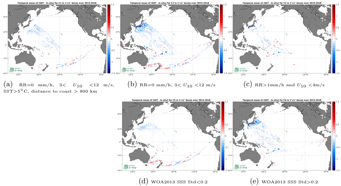
Figure 12: Temporal mean gridded over spatial boxes of size 1^\circ \times 1^\circ of \Delta SSS (SMAP-L3-RSS-V4-8DAY-RUNNING - TSG-LEGOS-DM) for 5 different subdatasets corresponding to:RR=0 mm/h, 3 < U_{10} < 12 m/s, SST >5^\circ C, distance to coast > 800 km (a), RR=0 mm/h, 3 < U_{10} < 12 m/s (b), RR >1 mm/h and U_{10} < 4 m/s (c), WOA2013 SSS Std <0.2 (d), WOA2013 SSS Std >0.2 (e).
