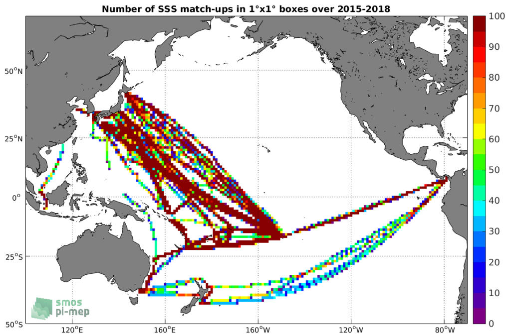
Figure 4: Number of SSS match-ups between TSG-LEGOS-DM SSS and the SMAP-L3-RSS-V4-8DAY-RUNNING SSS product for the Pacific Ocean Pi-MEP region over 1°x1° boxes and for the full satellite product period.
