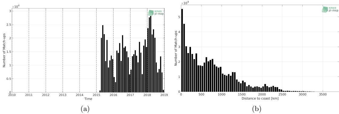
Figure 1: Number of match-ups between TSG-LEGOS-DM and SMAP-L3-RSS-V4-8DAY-RUNNING SSS as a function of time (a) and as function of the distance to coast (b) over the Pacific Ocean Pi-MEP region and for the full satellite product period.
