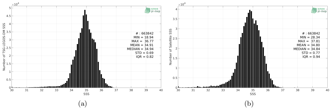
Figure 2: Histograms of SSS from TSG-LEGOS-DM (a) and SMAP-L3-RSS-V4-8DAY-RUNNING (b) considering all match-up pairs per bins of 0.1 over the Pacific Ocean Pi-MEP region and for the full satellite product period.
