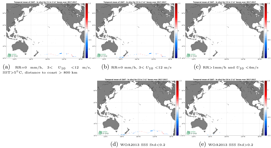
Figure 12: Temporal mean gridded over spatial boxes of size 1^{\circ}\times 1^{\circ} of \Delta SSS (SMAP-L3-RSS-V4-8DAY-RUNNING - TSG-GOSUD-Sailing-ship) for 5 different subdatasets corresponding to:RR=0 mm/h, 3 < U_{10} < 12 m/s, SST >5^{\circ}\text{C} , distance to coast > 800 km (a), RR=0 mm/h, 3 < U_{10} < 12 m/s (b), RR >1 mm/h and U_{10} < 4 m/s (c), WOA2013 SSS Std <0.2 (d), WOA2013 SSS Std >0.2 (e).
