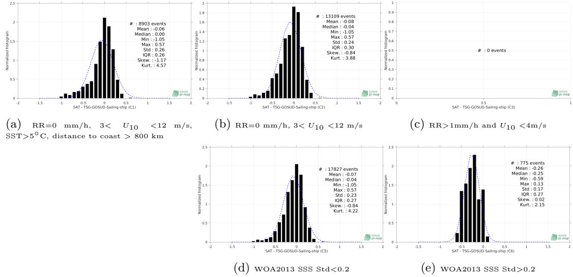
Figure 13: Normalized histogram of \Delta SSS (SMAP-L3-RSS-V4-8DAY-RUNNING - TSG-GOSUD-Sailing-ship) for 5 different subdatasets corresponding to: RR=0 mm/h, 3 < U_{10} < 12 m/s, SST > 5°C, distance to coast > 800 km (a), RR=0 mm/h, 3 < U_{10} < 12 m/s (b), RR > 1mm/h and U_{10} < 4 m/s (c), WOA2013 SSS Std < 0.2 (d), WOA2013 SSS Std > 0.2 (e).
