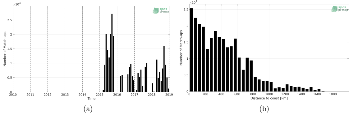
Figure 1: Number of match-ups between TSG-GOSUD-Research-vessel and SMAP-L3-RSS-V4-8DAY-RUNNING SSS as a function of time (a) and as function of the distance to coast (b) over the Pacific Ocean Pi-MEP region and for the full satellite product period.
