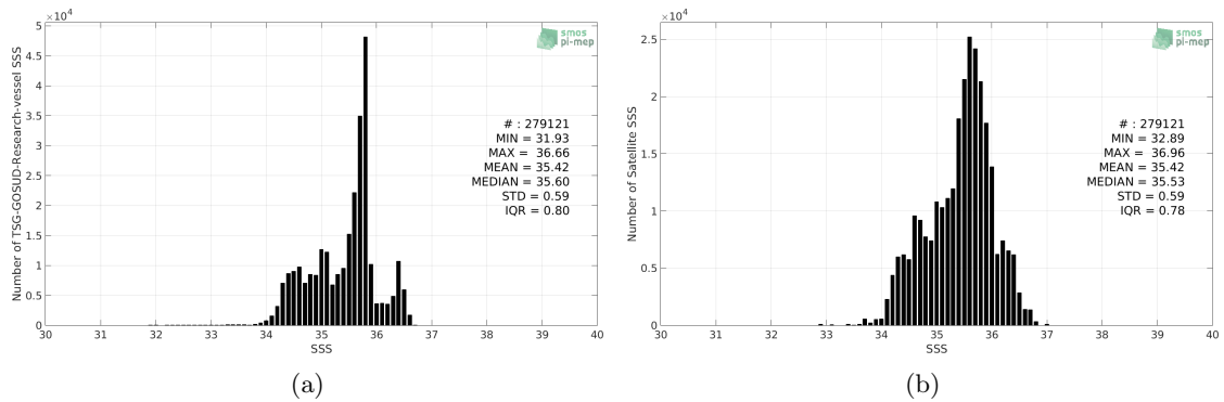
Figure 2: Histograms of SSS from TSG-GOSUD-Research-vessel (a) and SMAP-L3-RSS-V4-8DAY-RUNNING (b) considering all match-up pairs per bins of 0.1 over the Pacific Ocean Pi-MEP region and for the full satellite product period.
