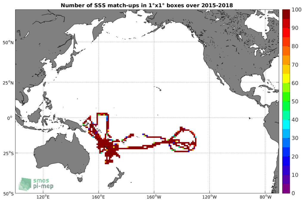
Figure 4: Number of SSS match-ups between TSG-GOSUD-Research-vessel SSS and the SMAP-L3-RSS-V4-8DAY-RUNNING SSS product for the Pacific Ocean Pi-MEP region over 1°x1° boxes and for the full satellite product period.
