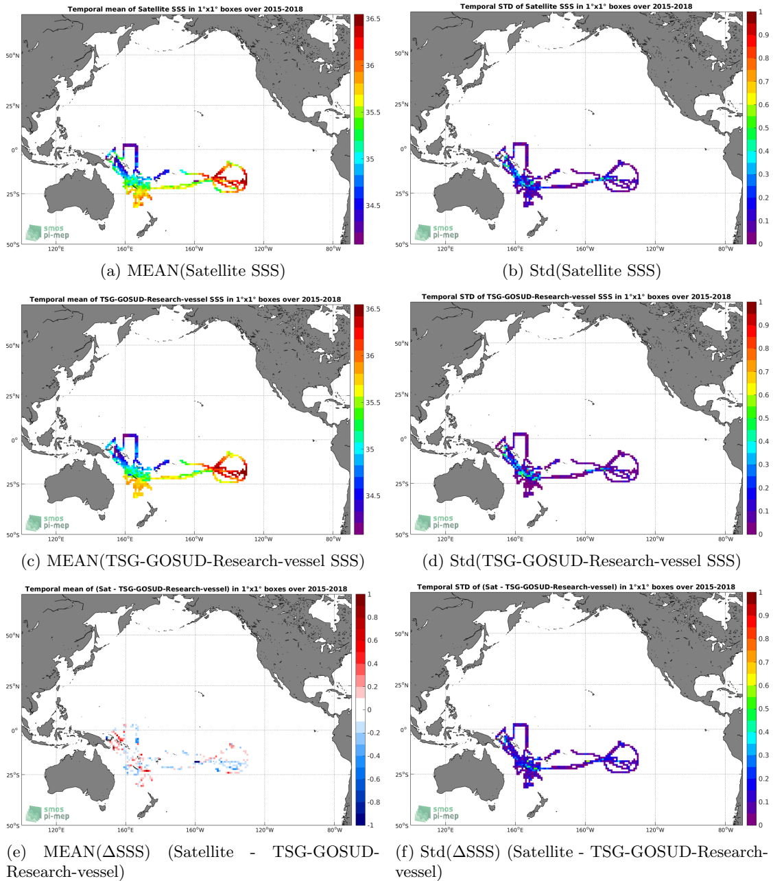
Figure 6: Temporal mean (left) and Std (right) of SSS from SMAP-L3-RSS-V4-8DAY-RUNNING (top), TSG-GOSUD-Research-vessel (middle), and of \Delta SSS (Satellite - TSG-GOSUD-Research-vessel). Only match-up pairs are used to generate these maps.
