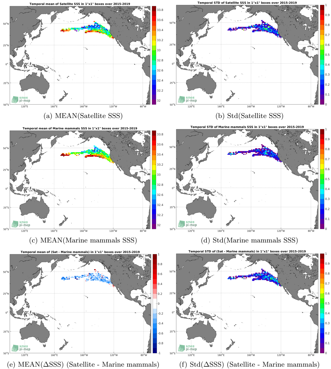
Figure 6: Temporal mean (left) and Std (right) of SSS from SMAP SSS L3 v4 - 8-Day running (RSS) (top), Marine mammals (middle), and of \Delta SSS (Satellite - Marine mammals). Only match-up pairs are used to generate these maps.
