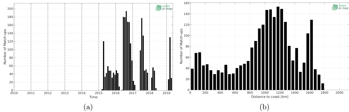
Figure 1: Number of match-ups between Marine mammals and SMAP SSS L3 v4 - 8-Day running (RSS) SSS as a function of time (a) and as function of the distance to coast (b) over the Pacific Ocean Pi-MEP region and for the full satellite product period.
