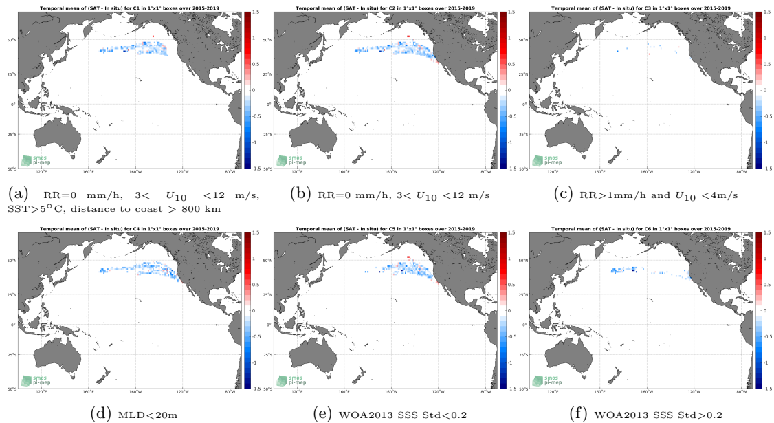
Figure 12: Temporal mean gridded over spatial boxes of size 1^\circ \times 1^\circ of \Delta SSS (SMAP SSS L3 v4 - 8-Day running (RSS) - Marine mammals) for 6 different subdatasets corresponding to:RR=0 mm/h, 3 < U_{10} < 12 m/s, SST > 5^\circ\text{C} , distance to coast > 800 km (a), RR=0 mm/h, 3 < U_{10} < 12 m/s (b), RR > 1 mm/h and U_{10} < 4 m/s (c),MLD < 20 m (d),WOA2013 SSS Std < 0.2 (e),WOA2013 SSS Std > 0.2 (f).
