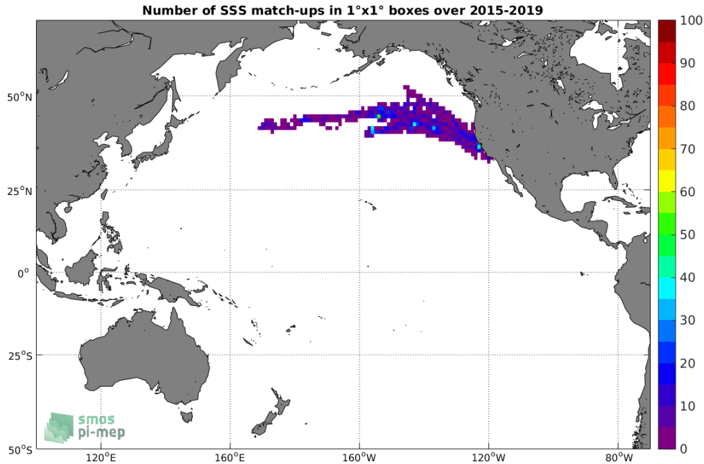
Figure 4: Number of SSS match-ups between Marine mammals SSS and the SMAP SSS L3 v4 - 8-Day running (RSS) SSS product for the Pacific Ocean Pi-MEP region over 1^\circ \times 1^\circ boxes and for the full satellite product period.
