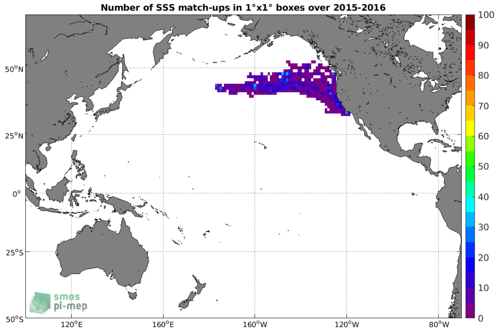
Figure 4: Number of SSS match-ups between Sea mammals SSS and the SMAP SSS L3 v4 - 8-Day running (RSS) SSS product for the Pacific Ocean Pi-MEP region over 1°x1° boxes and for the full satellite product period.
