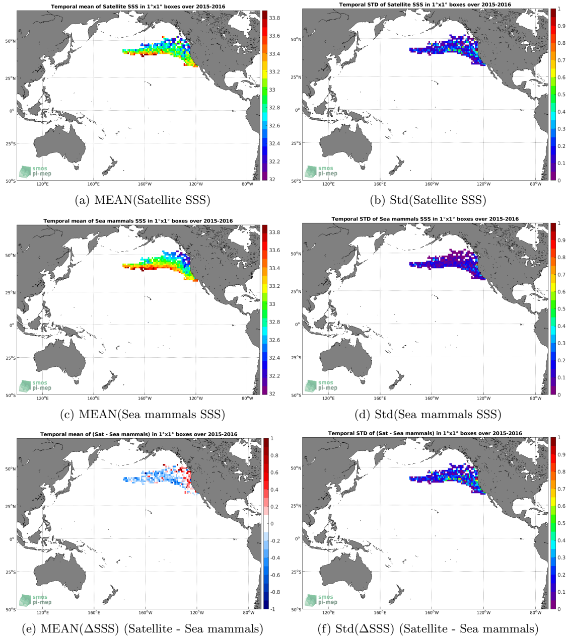
Figure 6: Temporal mean (left) and Std (right) of SSS from SMAP SSS L3 v4 - 8-Day running (RSS) (top), Sea mammals (middle), and of \Delta SSS (Satellite - Sea mammals). Only match-up pairs are used to generate these maps.
