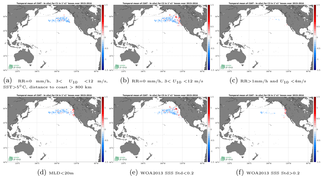
Figure 12: Temporal mean gridded over spatial boxes of size 1^\circ \times 1^\circ of \Delta SSS (SMAP SSS L3 v4 - 8-Day running (RSS) - Sea mammals) for 6 different subdatasets corresponding to:RR=0 mm/h, 3 < U_{10} < 12 m/s, SST >5^\circ C, distance to coast > 800 km (a), RR=0 mm/h, 3 < U_{10} < 12 m/s (b), RR >1 mm/h and U_{10} < 4 m/s (c),MLD <20 m (d),WOA2013 SSS Std <0.2 (e),WOA2013 SSS Std >0.2 (f).
