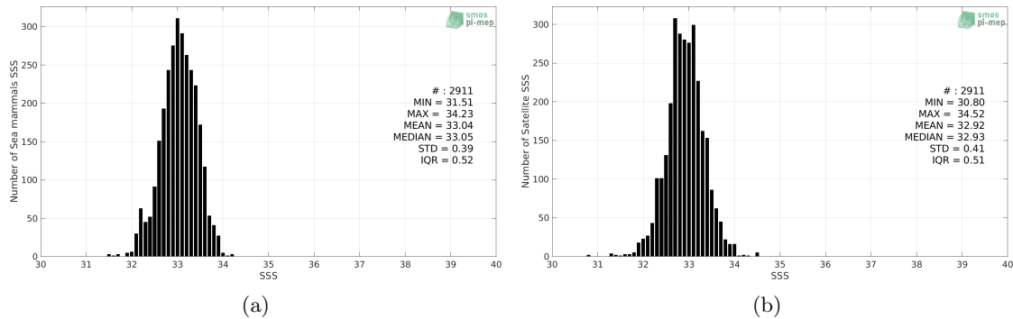
Figure 2: Histograms of SSS from Sea mammals (a) and SMAP SSS L3 v4 - 8-Day running (RSS) (b) considering all match-up pairs per bins of 0.1 over the Pacific Ocean Pi-MEP region and for the full satellite product period.
