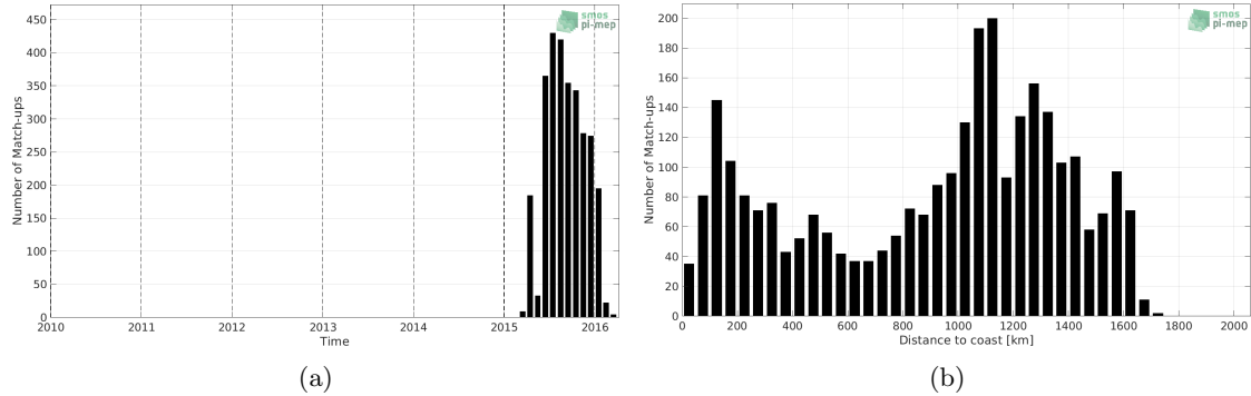
Figure 1: Number of match-ups between Sea mammals and SMAP SSS L3 v4 - 8-Day running (RSS) SSS as a function of time (a) and as function of the distance to coast (b) over the Pacific Ocean Pi-MEP region and for the full satellite product period.
