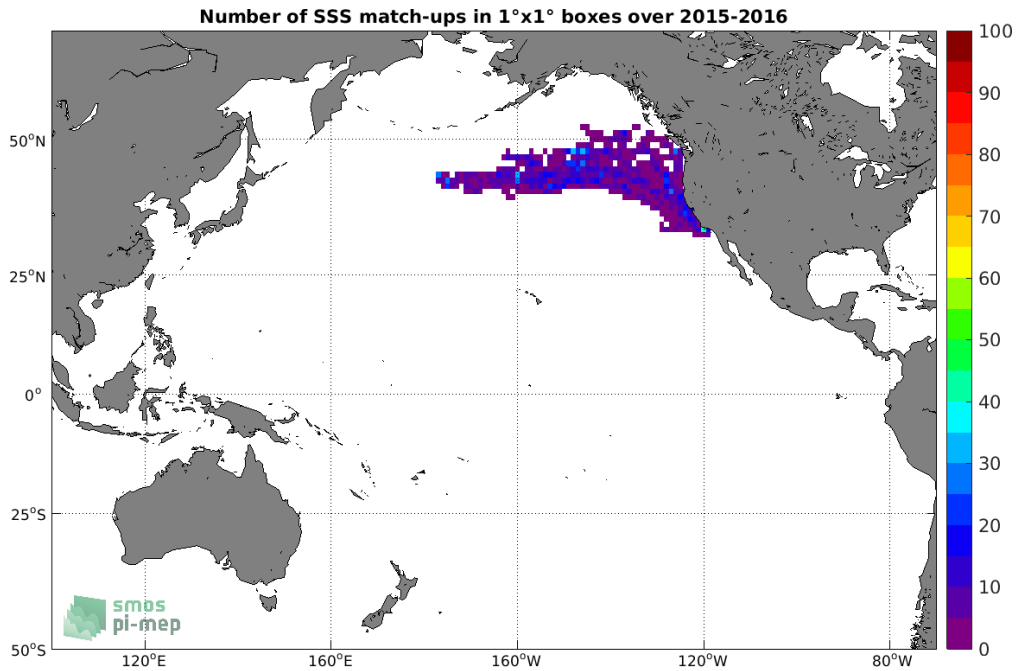
Figure 4: Number of SSS match-ups between Sea mammals SSS and the SMAP SSS L3 v4 - 8-Day running (RSS) SSS product for the Pacific Ocean Pi-MEP region over 1^\circ \times 1^\circ boxes and for the full satellite product period.
