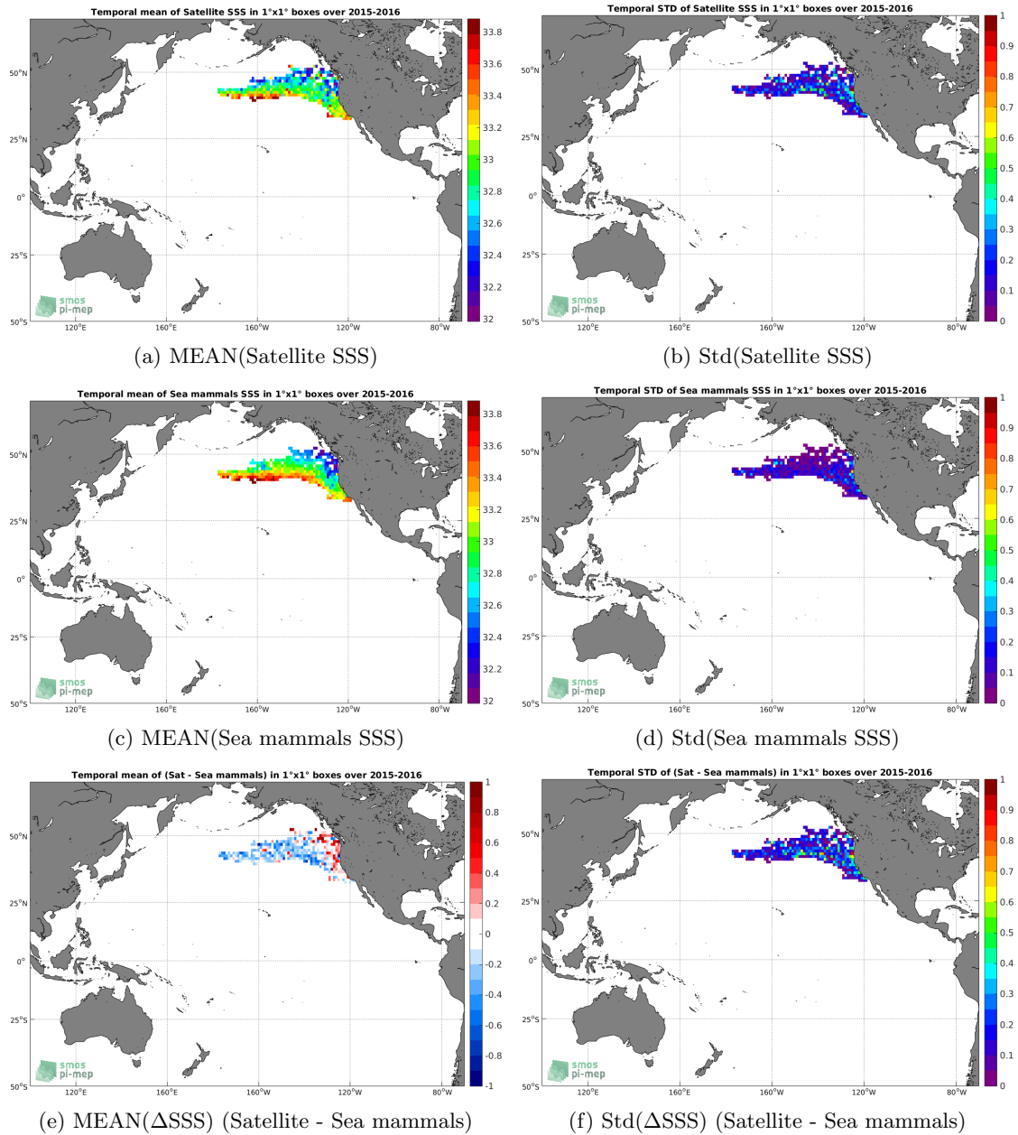
Figure 6: Temporal mean (left) and Std (right) of SSS from SMAP-L3-RSS-V4-8DAY-RUNNING (top), Sea mammals (middle), and of \Delta SSS (Satellite - Sea mammals). Only match-up pairs are used to generate these maps.
