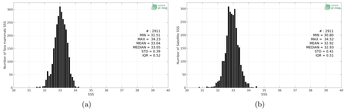
Figure 2: Histograms of SSS from Sea mammals (a) and SMAP-L3-RSS-V4-8DAY-RUNNING (b) considering all match-up pairs per bins of 0.1 over the Pacific Ocean Pi-MEP region and for the full satellite product period.
