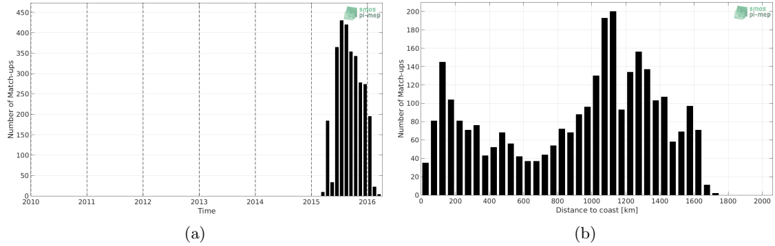
Figure 1: Number of match-ups between Sea mammals and SMAP-L3-RSS-V4-8DAY-RUNNING SSS as a function of time (a) and as function of the distance to coast (b) over the Pacific Ocean Pi-MEP region and for the full satellite product period.
