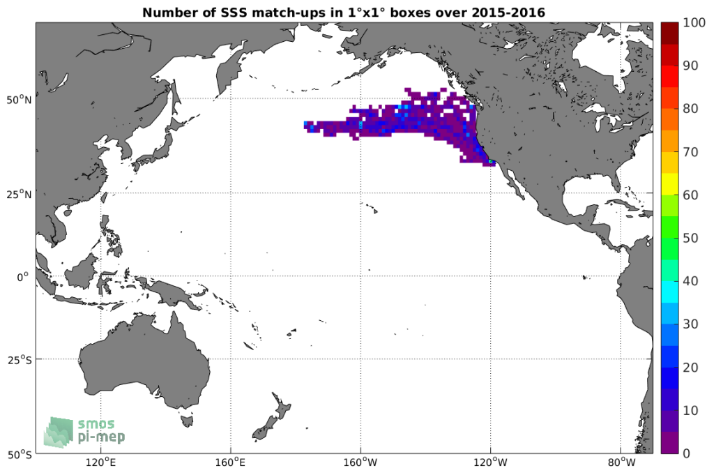
Figure 4: Number of SSS match-ups between Sea mammals SSS and the SMAP-L3-RSS-V4-8DAY-RUNNING SSS product for the Pacific Ocean Pi-MEP region over 1°x1° boxes and for the full satellite product period.
