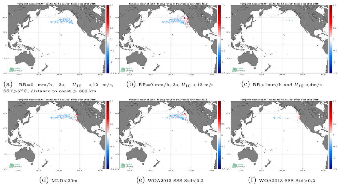
Figure 12: Temporal mean gridded over spatial boxes of size 1^\circ \times 1^\circ of \Delta SSS (SMAP-L3-RSS-V4-8DAY-RUNNING - Sea mammals) for 6 different subdatasets corresponding to:RR=0 mm/h, 3 < U_{10} < 12 m/s, SST >5^\circ C, distance to coast > 800 km (a), RR=0 mm/h, 3 < U_{10} < 12 m/s (b), RR >1 mm/h and U_{10} < 4 m/s (c),MLD <20 m (d),WOA2013 SSS Std <0.2 (e),WOA2013 SSS Std >0.2 (f).
