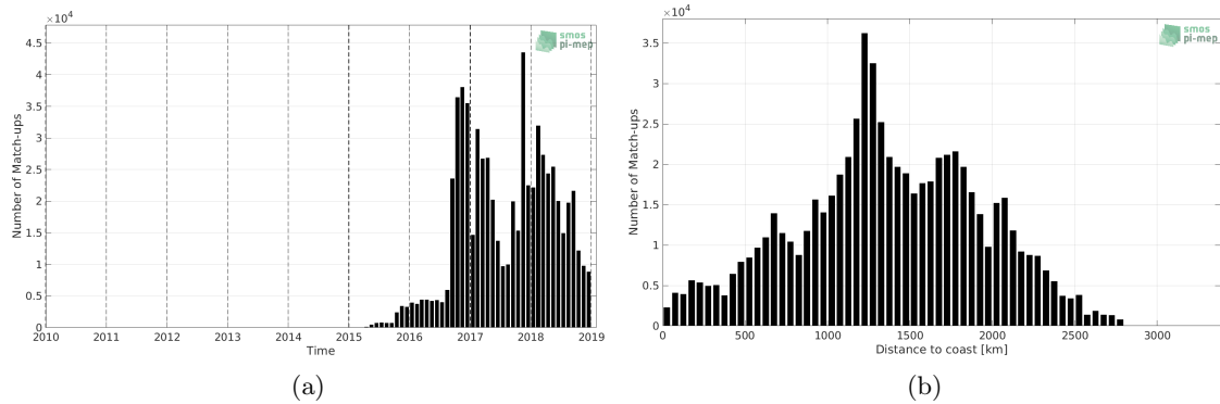
Figure 1: Number of match-ups between Surface drifters and SMAP SSS L3 v4 - 8-Day running (RSS) SSS as a function of time (a) and as function of the distance to coast (b) over the Pacific Ocean Pi-MEP region and for the full satellite product period.
