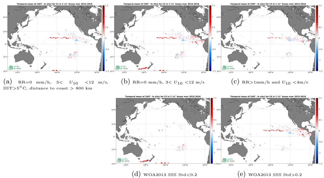
Figure 11: Temporal mean gridded over spatial boxes of size 1°x1° of \Delta SSS (SMAP SSS L3 v4 - 8-Day running (RSS) - Surface drifters) for 5 different subdatasets corresponding to:RR=0 mm/h, 3 < U_{10} < 12 m/s, SST > 5°C, distance to coast > 800 km (a), RR=0 mm/h, 3 < U_{10} < 12 m/s (b), RR > 1mm/h and U_{10} < 4 m/s (c), WOA2013 SSS Std < 0.2 (d), WOA2013 SSS Std > 0.2 (e).
