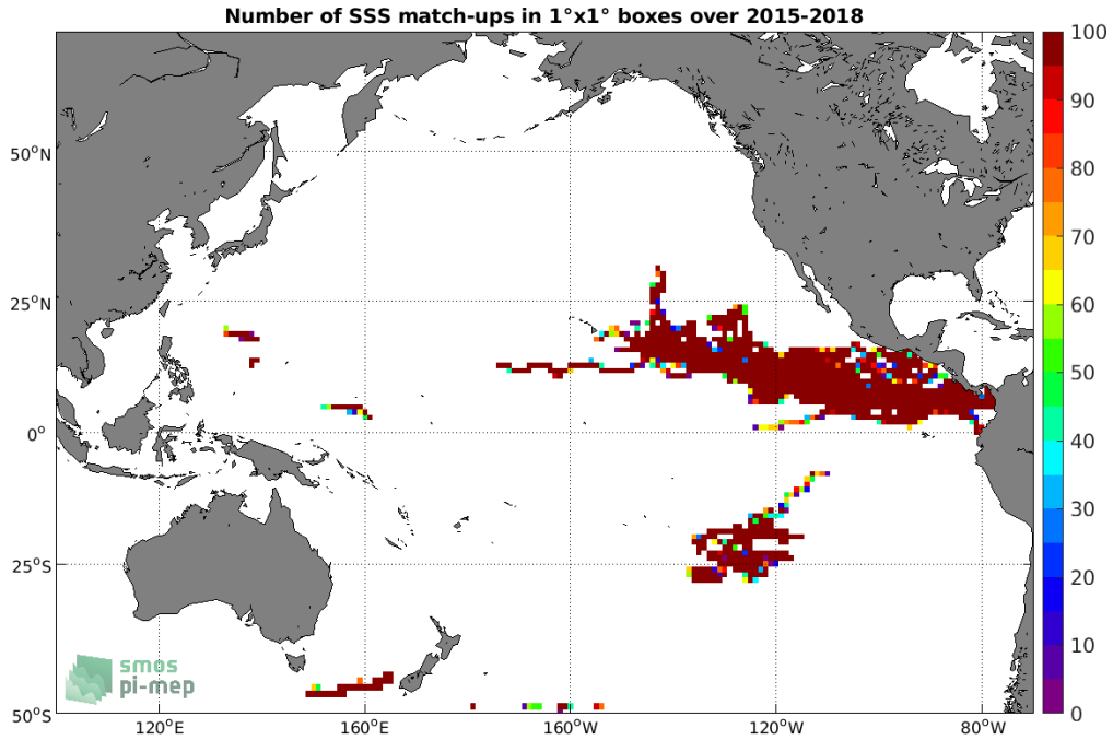
Figure 3: Number of SSS match-ups between Surface drifters SSS and the SMAP SSS L3 v4 - 8-Day running (RSS) SSS product for the Pacific Ocean Pi-MEP region over 1^\circ \times 1^\circ boxes and for the full satellite product period.
