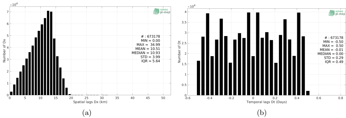
Figure 4: Histograms of the spatial (a) and temporal (b) lags between the location/time of the Surface drifters measurement and the date of the corresponding SMAP SSS L3 v4 - 8-Day running (RSS) SSS pixel.
