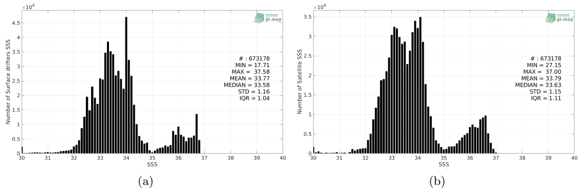
Figure 2: Histograms of SSS from Surface drifters (a) and SMAP SSS L3 v4 - 8-Day running (RSS) (b) considering all match-up pairs per bins of 0.1 over the Pacific Ocean Pi-MEP region and for the full satellite product period.
