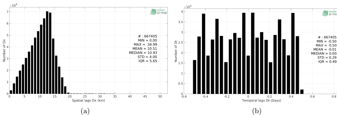
Figure 4: Histograms of the spatial (a) and temporal (b) lags between the time of the Surface drifters measurements and the date of the corresponding SMAP-L3-RSS-V4-8DAY-RUNNING SSS product.
