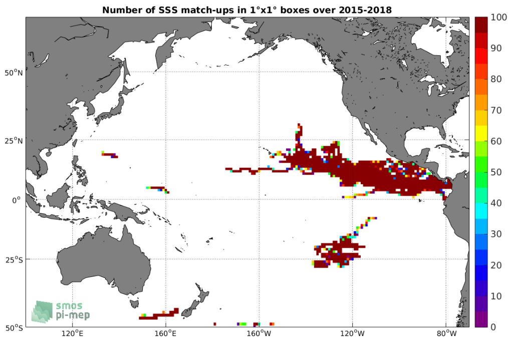
Figure 3: Number of SSS match-ups between Surface drifters SSS and the SMAP-L3-RSS-V4-8DAY-RUNNING SSS product for the Pacific Ocean Pi-MEP region over 1^{\circ} \times 1^{\circ} boxes and for the full satellite product period.
