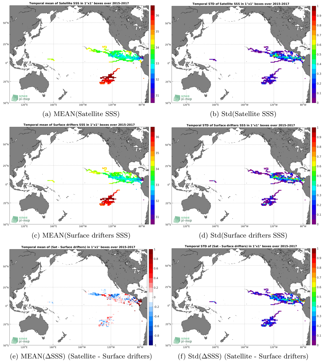
Figure 5: Temporal mean (left) and Std (right) of SSS from SMAP-L3-RSS-V4-8DAY-RUNNING (top), Surface drifters (middle), and of \Delta SSS (Satellite - Surface drifters). Only match-up pairs are used to generate these maps.
