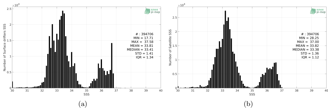
Figure 2: Histograms of SSS from Surface drifters (a) and SMAP-L3-RSS-V4-8DAY-RUNNING (b) considering all match-up pairs per bins of 0.1 over the Pacific Ocean Pi-MEP region and for the full satellite product period.
