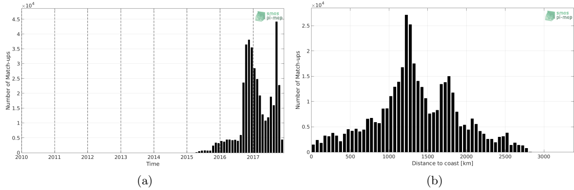
Figure 1: Number of match-ups between Surface drifters and SMAP-L3-RSS-V4-8DAY-RUNNING SSS as a function of time (a) and as function of the distance to coast (b) over the Pacific Ocean Pi-MEP region and for the full satellite product period.
