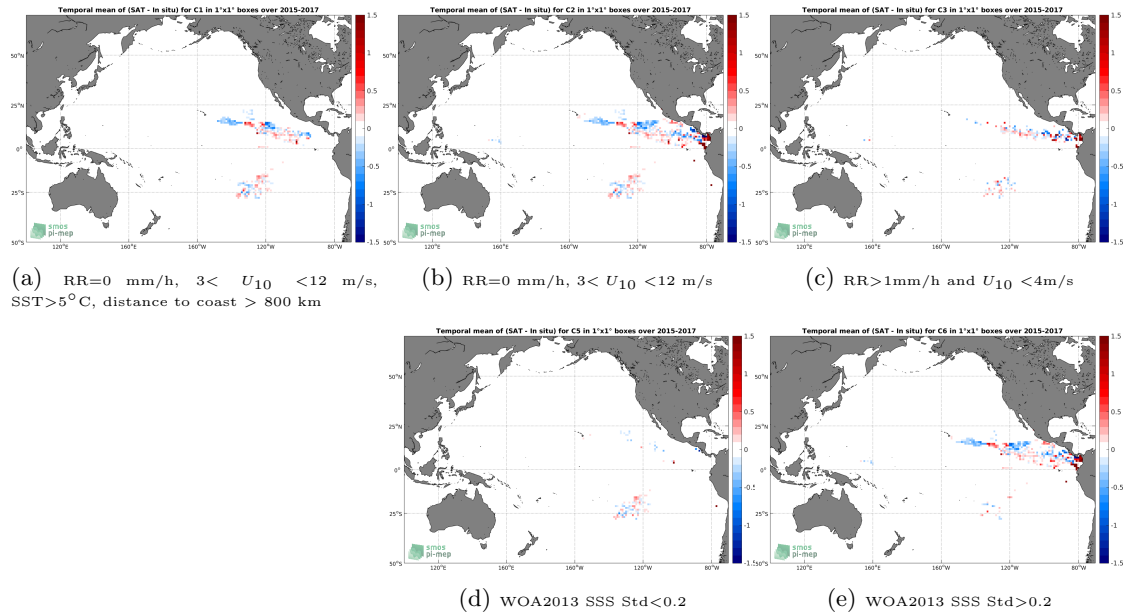
Figure 11: Temporal mean gridded over spatial boxes of size 1^\circ \times 1^\circ of \Delta SSS (SMAP-L3-RSS-V4-8DAY-RUNNING - Surface drifters) for 5 different subdatasets corresponding to:RR=0 mm/h, 3 < U_{10} < 12 m/s, SST >5^\circ\text{C} , distance to coast > 800 km (a), RR=0 mm/h, 3 < U_{10} < 12 m/s (b), RR >1 mm/h and U_{10} < 4 m/s (c), WOA2013 SSS Std <0.2 (d), WOA2013 SSS Std >0.2 (e).
