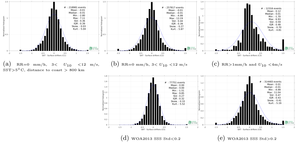
Figure 12: Normalized histogram of \Delta SSS (SMAP-L3-RSS-V4-8DAY-RUNNING - Surface drifters) for 5 different subdatasets corresponding to: RR=0 mm/h, 3 < U_{10} < 12 m/s, SST > 5°C, distance to coast > 800 km (a), RR=0 mm/h, 3 < U_{10} < 12 m/s (b), RR > 1mm/h and U_{10} < 4 m/s (c), WOA2013 SSS Std < 0.2 (d), WOA2013 SSS Std > 0.2 (e).
