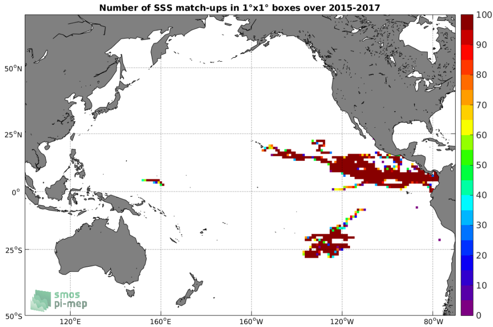
Figure 3: Number of SSS match-ups between Surface drifters SSS and the SMAP-L3-RSS-V4-8DAY-RUNNING SSS product for the Pacific Ocean Pi-MEP region over 1^\circ \times 1^\circ boxes and for the full satellite product period.
