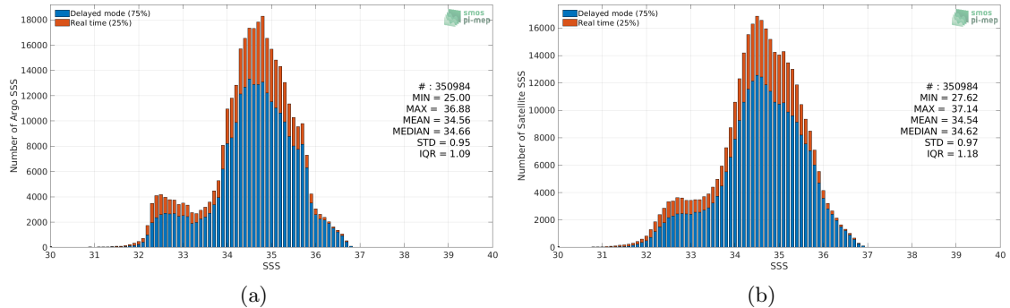
Figure 2: Histograms of SSS from Argo (a) and SMAP SSS L3 v4 - 8-Day running (RSS) (b) considering all match-up pairs per bins of 0.1 over the Pacific Ocean Pi-MEP region and for the full satellite product period.
