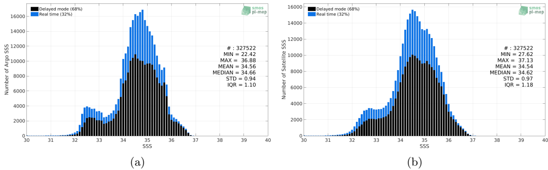
Figure 2: Histograms of SSS from Argo (a) and SMAP SSS L3 v4 - 8-Day running (RSS) (b) considering all match-up pairs per bins of 0.1 over the Pacific Ocean Pi-MEP region and for the full satellite product period.
