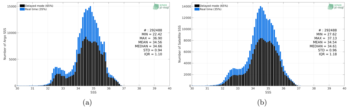
Figure 2: Histograms of SSS from Argo (a) and SMAP-L3-RSS-V4-8DAY-RUNNING (b) considering all match-up pairs per bins of 0.1 over the Pacific Ocean Pi-MEP region and for the full satellite product period.
