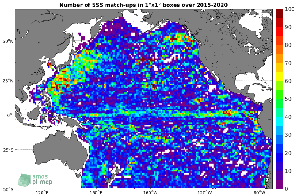
Figure 4: Number of SSS match-ups between Argo SSS and the SMAP-L3-RSS-V4-8DAY-RUNNING SSS product for the Pacific Ocean Pi-MEP region over 1^\circ \times 1^\circ boxes and for the full satellite product period.
