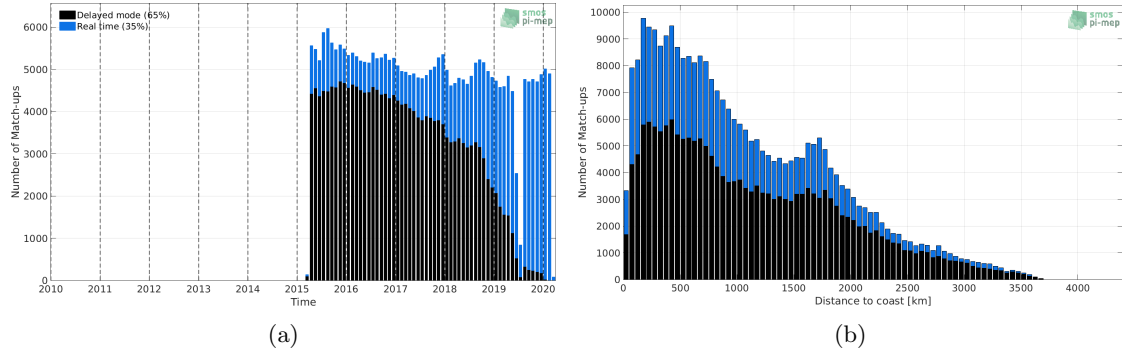
Figure 1: Number of match-ups between Argo and SMAP-L3-RSS-V4-8DAY-RUNNING SSS as a function of time (a) and as function of the distance to coast (b) over the Pacific Ocean Pi-MEP region and for the full satellite product period.
