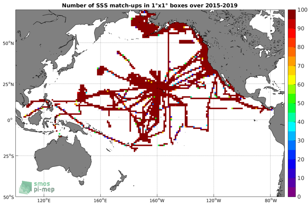
Figure 4: Number of SSS match-ups between TSG-SAMOS SSS and the SMAP-L3-RSS-V4-MONTHLY SSS product for the Pacific Ocean Pi-MEP region over 1^\circ \times 1^\circ boxes and for the full satellite product period.
