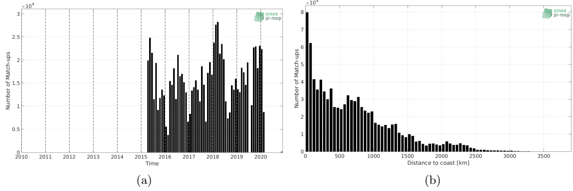
Figure 1: Number of match-ups between TSG (LEGOS-DM) and SMAP SSS L3 v4 - Monthly (RSS) SSS as a function of time (a) and as function of the distance to coast (b) over the Pacific Ocean Pi-MEP region and for the full satellite product period.
