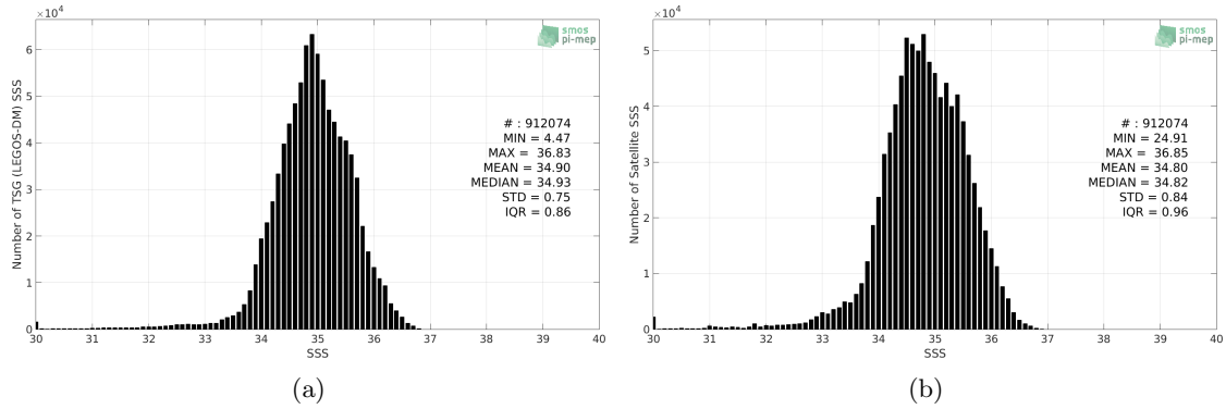
Figure 2: Histograms of SSS from TSG (LEGOS-DM) (a) and SMAP SSS L3 v4 - Monthly (RSS) (b) considering all match-up pairs per bins of 0.1 over the Pacific Ocean Pi-MEP region and for the full satellite product period.
