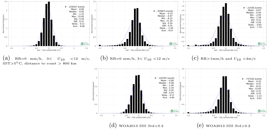
Figure 13: Normalized histogram of \Delta\text{SSS} (SMAP SSS L3 v4 - Monthly (RSS) - TSG (LEGOS-DM)) for 5 different subdatasets corresponding to: RR=0 mm/h, 3 < U_{10} < 12 m/s, SST>5°C, distance to coast > 800 km (a), RR=0 mm/h, 3 < U_{10} < 12 m/s (b), RR>1mm/h and U_{10} < 4 m/s (c), WOA2013 SSS Std<0.2 (d), WOA2013 SSS Std>0.2 (e).
