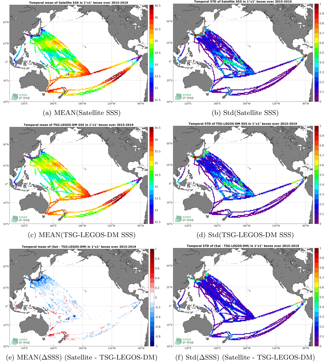
Figure 6: Temporal mean (left) and Std (right) of SSS from SMAP-L3-RSS-V4-MONTHLY (top), TSG-LEGOS-DM (middle), and of \Delta SSS (Satellite - TSG-LEGOS-DM). Only match-up pairs are used to generate these maps.
