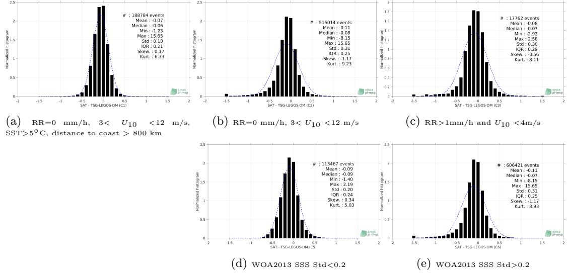
Figure 13: Normalized histogram of \Delta SSS (SMAP-L3-RSS-V4-MONTHLY - TSG-LEGOS-DM) for 5 different subdatasets corresponding to: RR=0 mm/h, 3 < U_{10} < 12 m/s, SST > 5°C, distance to coast > 800 km (a), RR=0 mm/h, 3 < U_{10} < 12 m/s (b), RR > 1mm/h and U_{10} < 4 m/s (c), WOA2013 SSS Std < 0.2 (d), WOA2013 SSS Std > 0.2 (e).
