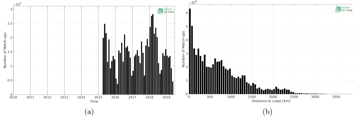
Figure 1: Number of match-ups between TSG-LEGOS-DM and SMAP-L3-RSS-V4-MONTHLY SSS as a function of time (a) and as function of the distance to coast (b) over the Pacific Ocean Pi-MEP region and for the full satellite product period.
