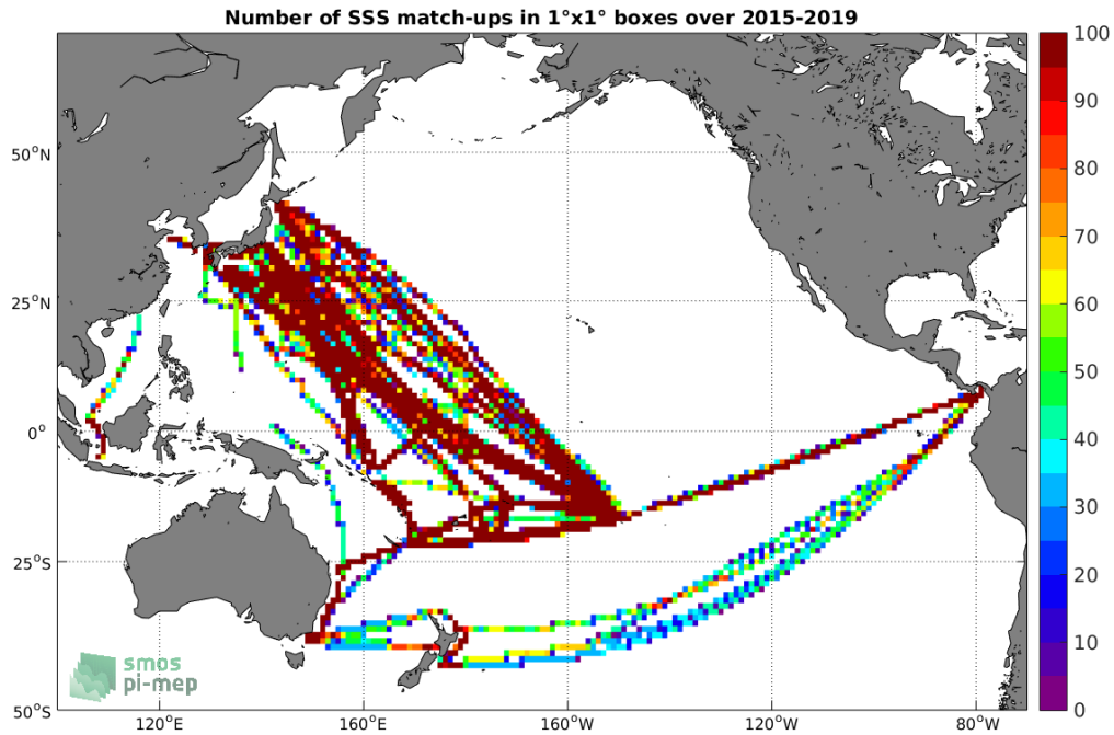
Figure 4: Number of SSS match-ups between TSG-LEGOS-DM SSS and the SMAP-L3-RSS-V4-MONTHLY SSS product for the Pacific Ocean Pi-MEP region over 1°x1° boxes and for the full satellite product period.
