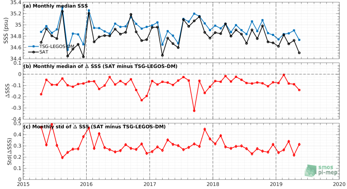
Figure 7: Time series of the monthly median SSS (top), median of \Delta\text{SSS} (Satellite - TSG-LEGOS-DM) and Std of \Delta\text{SSS} (Satellite - TSG-LEGOS-DM) over the Pacific Ocean Pi-MEP region considering all match-ups collected by the Pi-MEP.
