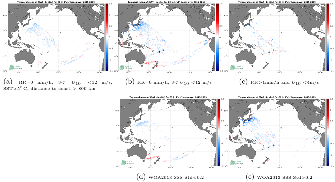
Figure 12: Temporal mean gridded over spatial boxes of size 1^\circ \times 1^\circ of \Delta SSS (SMAP-L3-RSS-V4-MONTHLY - TSG-LEGOS-DM) for 5 different subdatasets corresponding to: RR=0 mm/h, 3 < U_{10} < 12 m/s, SST > 5^\circ C , distance to coast > 800 km (a), RR=0 mm/h, 3 < U_{10} < 12 m/s (b), RR > 1 mm/h and U_{10} < 4 m/s (c), WOA2013 SSS Std < 0.2 (d), WOA2013 SSS Std > 0.2 (e).
