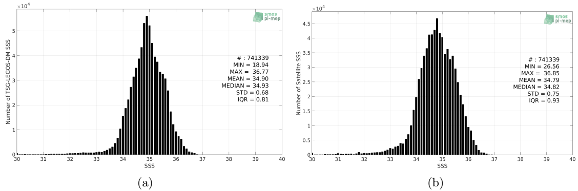
Figure 2: Histograms of SSS from TSG-LEGOS-DM (a) and SMAP-L3-RSS-V4-MONTHLY (b) considering all match-up pairs per bins of 0.1 over the Pacific Ocean Pi-MEP region and for the full satellite product period.
