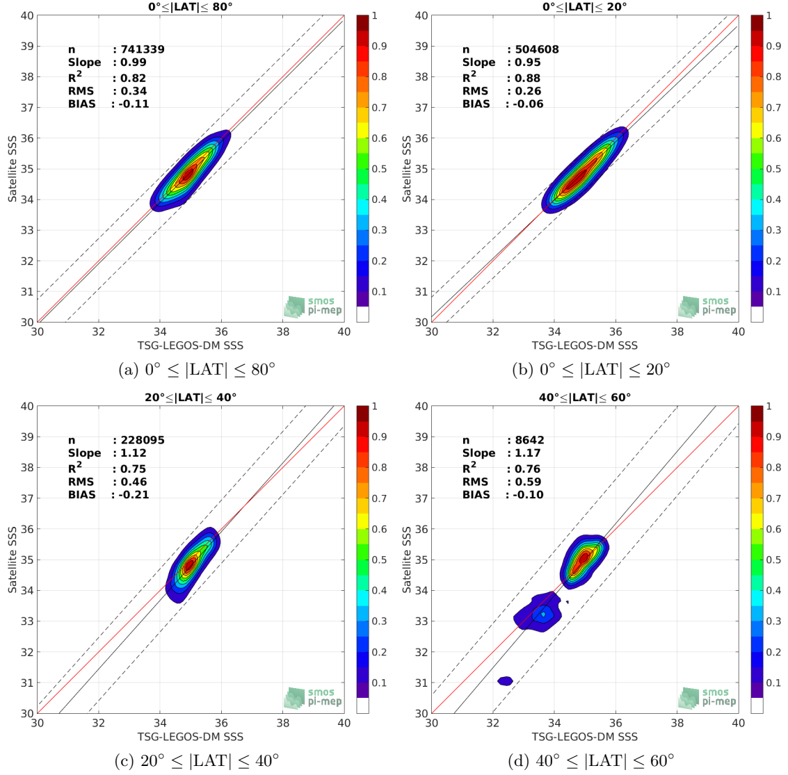
Figure 9: Contour maps of the concentration of SMAP-L3-RSS-V4-MONTHLY SSS (y-axis) versus TSG-LEGOS-DM SSS (x-axis) at match-up pairs for different latitude bands. For each plot, the red line shows x=y . The black thin and dashed lines indicate a linear fit through the data cloud and the \pm 95\% confidence levels, respectively. The number match-up pairs n , the slope and R^2 coefficient of the linear fit, the root mean square (RMS) and the mean bias between satellite and in situ data are indicated for each latitude band in each plots.
