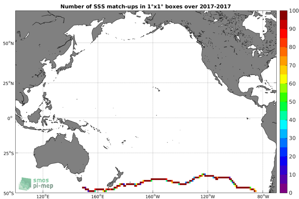
Figure 4: Number of SSS match-ups between TSG-GOSUD-Sailing-ship SSS and the SMAP-L3-RSS-V4-MONTHLY SSS product for the Pacific Ocean Pi-MEP region over 1°x1° boxes and for the full satellite product period.
