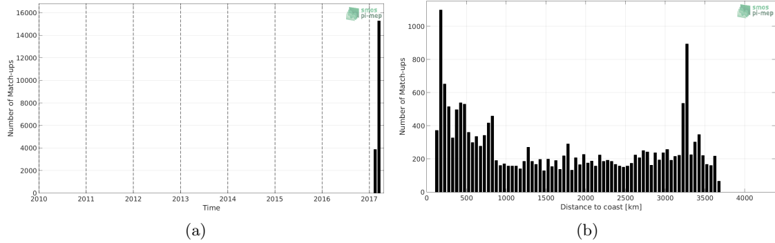
Figure 1: Number of match-ups between TSG-GOSUD-Sailing-ship and SMAP-L3-RSS-V4-MONTHLY SSS as a function of time (a) and as function of the distance to coast (b) over the Pacific Ocean Pi-MEP region and for the full satellite product period.
