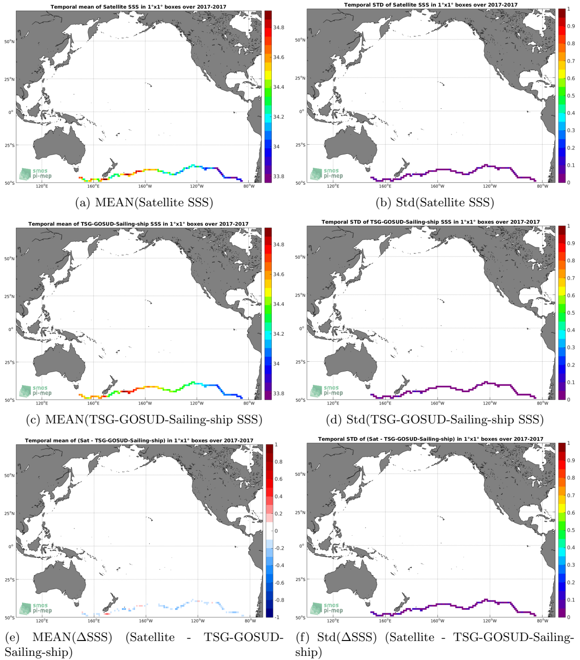
Figure 6: Temporal mean (left) and Std (right) of SSS from SMAP-L3-RSS-V4-MONTHLY (top), TSG-GOSUD-Sailing-ship (middle), and of \Delta SSS (Satellite - TSG-GOSUD-Sailing-ship). Only match-up pairs are used to generate these maps.
