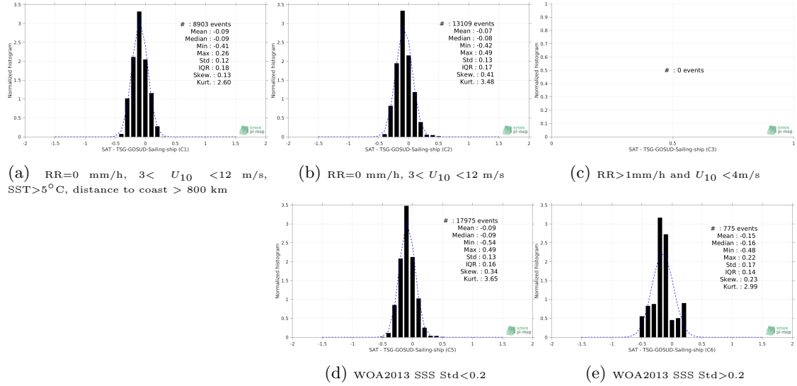
Figure 13: Normalized histogram of \Delta SSS (SMAP-L3-RSS-V4-MONTHLY - TSG-GOSUD-Sailing-ship) for 5 different subdatasets corresponding to: RR=0 mm/h, 3 < U_{10} < 12 m/s, SST>5°C, distance to coast > 800 km (a), RR=0 mm/h, 3 < U_{10} < 12 m/s (b), RR>1mm/h and U_{10} < 4 m/s (c), WOA2013 SSS Std<0.2 (d), WOA2013 SSS Std>0.2 (e).
