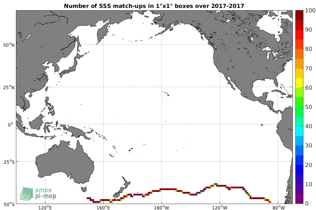
Figure 4: Number of SSS match-ups between TSG-GOSUD-Sailing-ship SSS and the SMAP-L3-RSS-V4-MONTHLY SSS product for the Pacific Ocean Pi-MEP region over 1^\circ \times 1^\circ boxes and for the full satellite product period.
