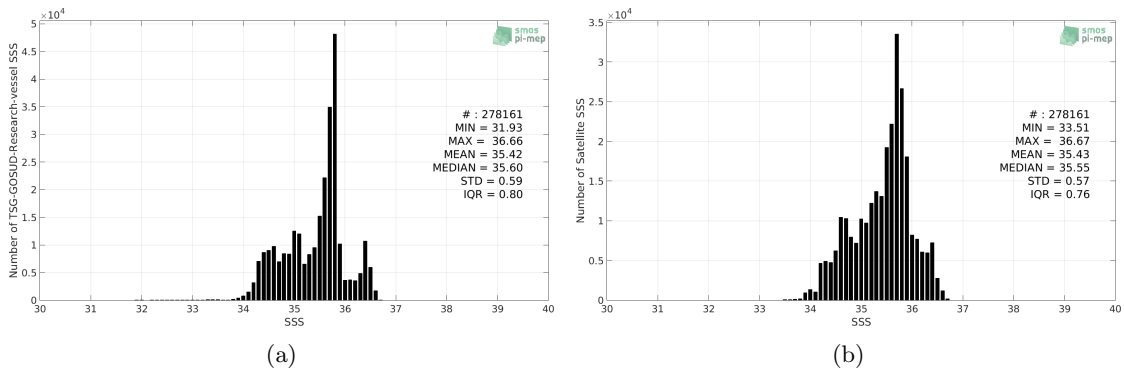
Figure 2: Histograms of SSS from TSG-GOSUD-Research-vessel (a) and SMAP-L3-RSS-V4-MONTHLY (b) considering all match-up pairs per bins of 0.1 over the Pacific Ocean Pi-MEP region and for the full satellite product period.
