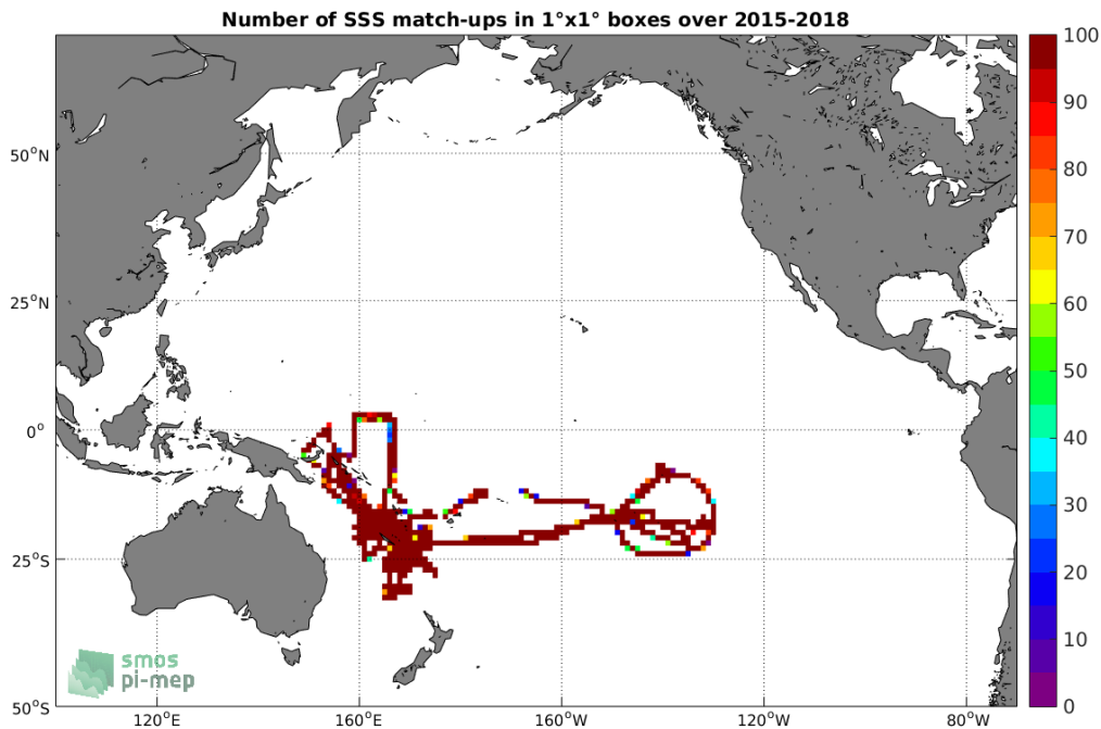
Figure 4: Number of SSS match-ups between TSG-GOSUD-Research-vessel SSS and the SMAP-L3-RSS-V4-MONTHLY SSS product for the Pacific Ocean Pi-MEP region over 1^\circ \times 1^\circ boxes and for the full satellite product period.
