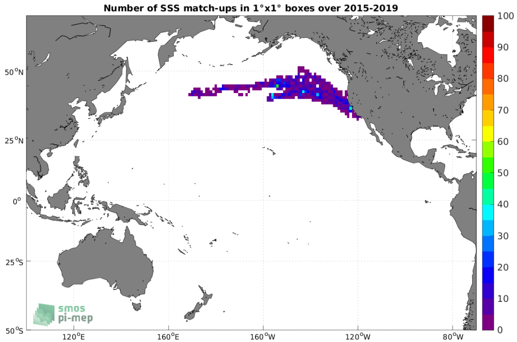
Figure 4: Number of SSS match-ups between Marine mammals SSS and the SMAP SSS L3 v4 - Monthly (RSS) SSS product for the Pacific Ocean Pi-MEP region over 1^\circ \times 1^\circ boxes and for the full satellite product period.
