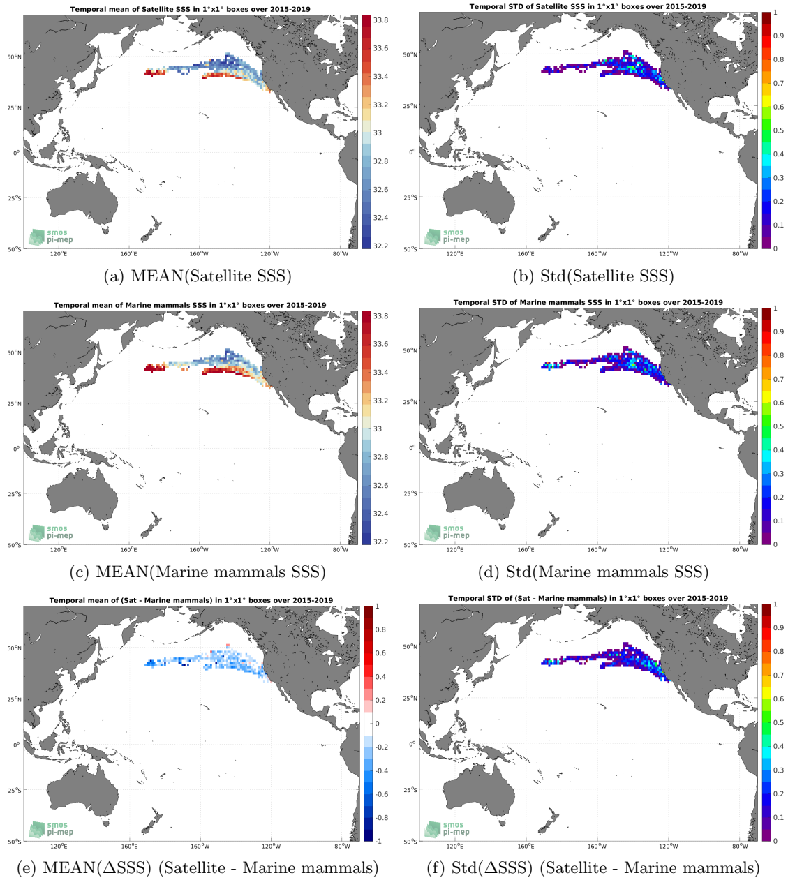
Figure 6: Temporal mean (left) and Std (right) of SSS from SMAP SSS L3 v4 - Monthly (RSS) (top), Marine mammals (middle), and of \Delta SSS (Satellite - Marine mammals). Only match-up pairs are used to generate these maps.
