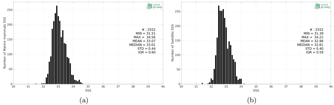
Figure 2: Histograms of SSS from Marine mammals (a) and SMAP SSS L3 v4 - Monthly (RSS) (b) considering all match-up pairs per bins of 0.1 over the Pacific Ocean Pi-MEP region and for the full satellite product period.
