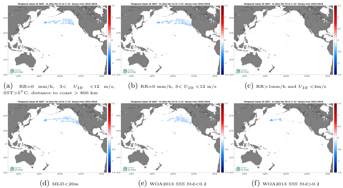
Figure 12: Temporal mean gridded over spatial boxes of size 1^\circ \times 1^\circ of \Delta SSS (SMAP SSS L3 v4 - Monthly (RSS) - Marine mammals) for 6 different subdatasets corresponding to:RR=0 mm/h, 3 < U_{10} < 12 m/s, SST > 5^\circ\text{C} , distance to coast > 800 km (a), RR=0 mm/h, 3 < U_{10} < 12 m/s (b), RR > 1 mm/h and U_{10} < 4 m/s (c),MLD < 20 m (d),WOA2013 SSS Std < 0.2 (e),WOA2013 SSS Std > 0.2 (f).
