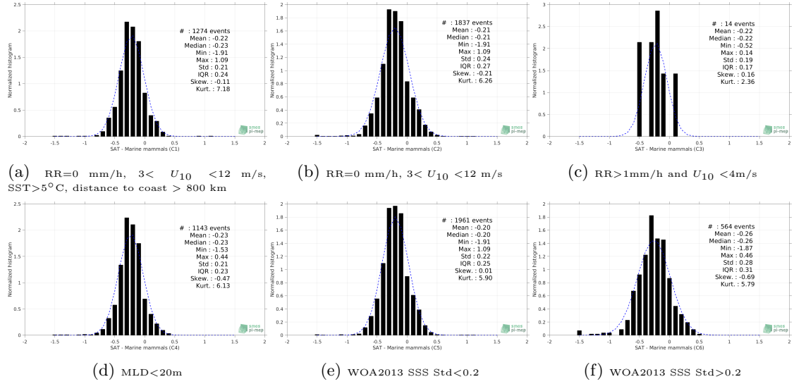
Figure 13: Normalized histogram of \Delta SSS (SMAP SSS L3 v4 - Monthly (RSS) - Marine mammals) for 6 different subdatasets corresponding to: RR=0 mm/h, 3 < U_{10} < 12 m/s, SST > 5°C, distance to coast > 800 km (a), RR=0 mm/h, 3 < U_{10} < 12 m/s (b), RR > 1mm/h and U_{10} < 4 m/s (c), MLD < 20m (d), WOA2013 SSS Std < 0.2 (e), WOA2013 SSS Std > 0.2 (f).
