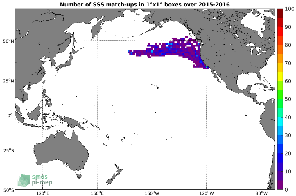
Figure 4: Number of SSS match-ups between Sea mammals SSS and the SMAP SSS L3 v4 - Monthly (RSS) SSS product for the Pacific Ocean Pi-MEP region over 1°x1° boxes and for the full satellite product period.
