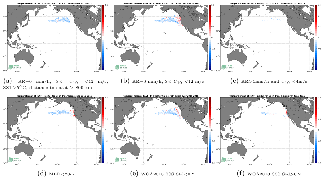
Figure 12: Temporal mean gridded over spatial boxes of size 1^\circ \times 1^\circ of \Delta SSS (SMAP SSS L3 v4 - Monthly (RSS) - Sea mammals) for 6 different subdatasets corresponding to:RR=0 mm/h, 3 < U_{10} < 12 m/s, SST>5°C, distance to coast > 800 km (a), RR=0 mm/h, 3 < U_{10} < 12 m/s (b), RR>1mm/h and U_{10} < 4 m/s (c),MLD<20m (d),WOA2013 SSS Std<0.2 (e),WOA2013 SSS Std>0.2 (f).
