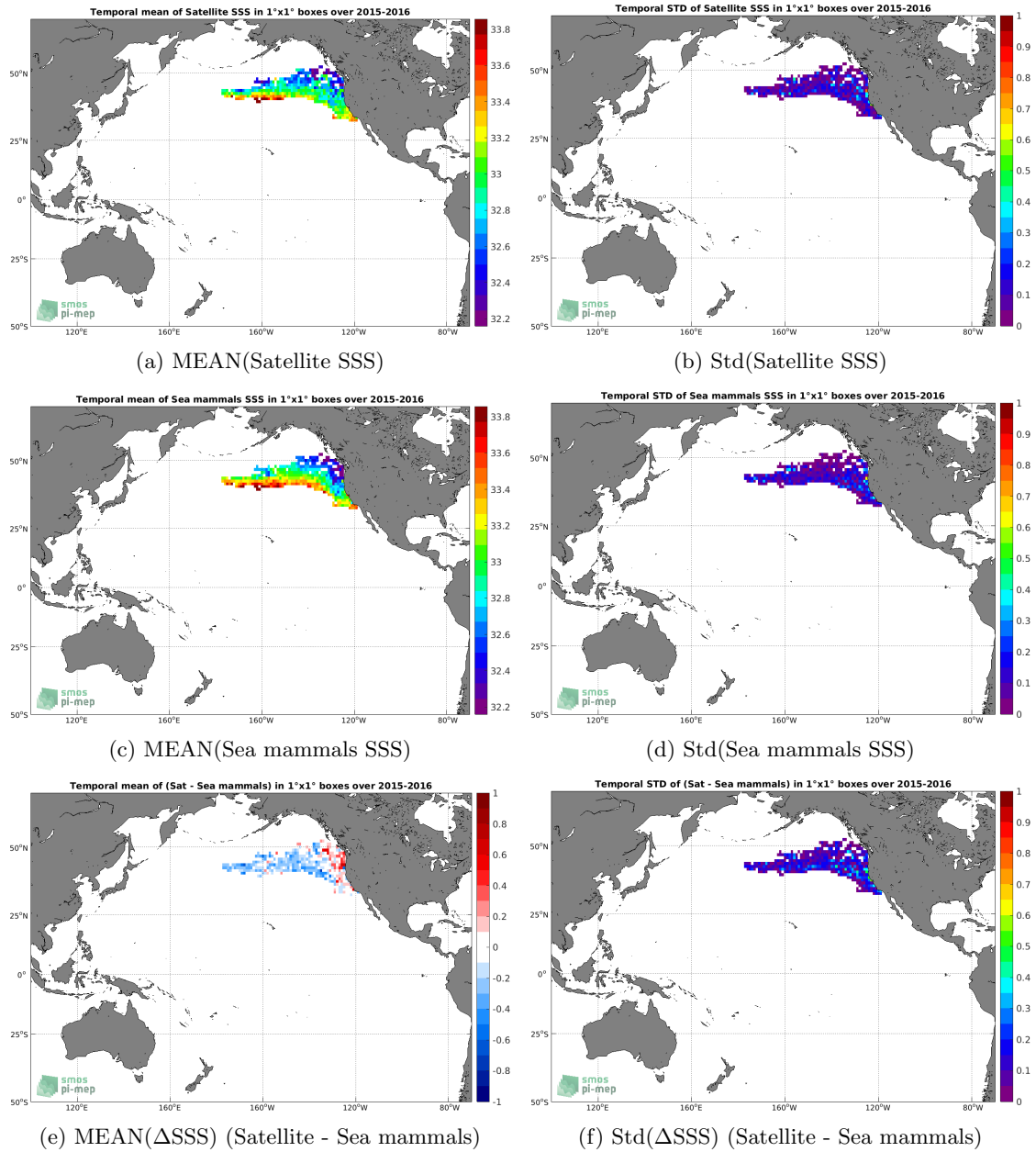
Figure 6: Temporal mean (left) and Std (right) of SSS from SMAP SSS L3 v4 - Monthly (RSS) (top), Sea mammals (middle), and of \Delta SSS (Satellite - Sea mammals). Only match-up pairs are used to generate these maps.
