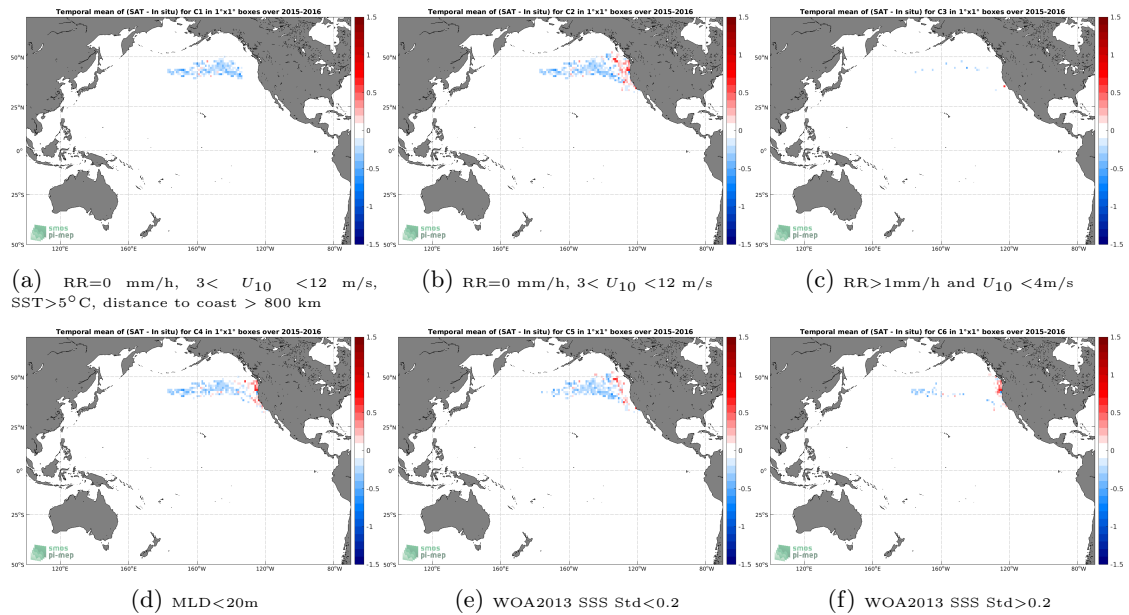
Figure 12: Temporal mean gridded over spatial boxes of size 1°x1° of \Delta SSS (SMAP SSS L3 v4 - Monthly (RSS) - Sea mammals) for 6 different subdatasets corresponding to:RR=0 mm/h, 3 < U_{10} < 12 m/s, SST>5°C, distance to coast > 800 km (a), RR=0 mm/h, 3 < U_{10} < 12 m/s (b), RR>1mm/h and U_{10} < 4 m/s (c),MLD<20m (d),WOA2013 SSS Std<0.2 (e),WOA2013 SSS Std>0.2 (f).
