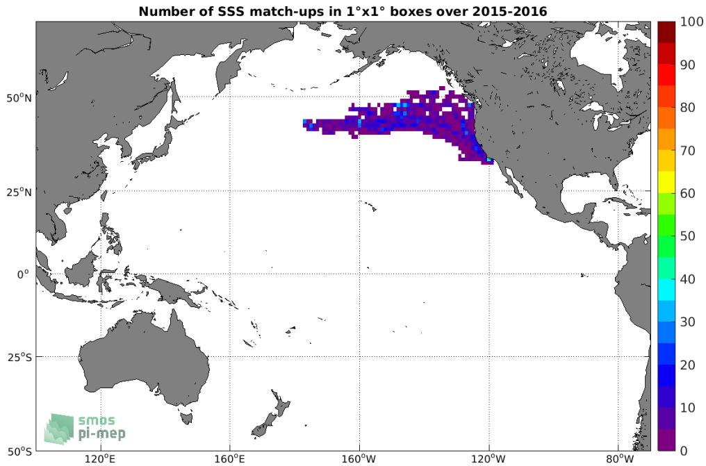
Figure 4: Number of SSS match-ups between Sea mammals SSS and the SMAP SSS L3 v4 - Monthly (RSS) SSS product for the Pacific Ocean Pi-MEP region over 1^\circ \times 1^\circ boxes and for the full satellite product period.
