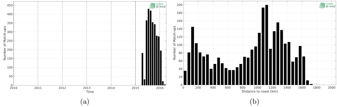
Figure 1: Number of match-ups between Sea mammals and SMAP SSS L3 v4 - Monthly (RSS) SSS as a function of time (a) and as function of the distance to coast (b) over the Pacific Ocean Pi-MEP region and for the full satellite product period.
