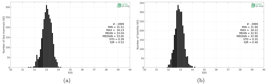
Figure 2: Histograms of SSS from Sea mammals (a) and SMAP SSS L3 v4 - Monthly (RSS) (b) considering all match-up pairs per bins of 0.1 over the Pacific Ocean Pi-MEP region and for the full satellite product period.
